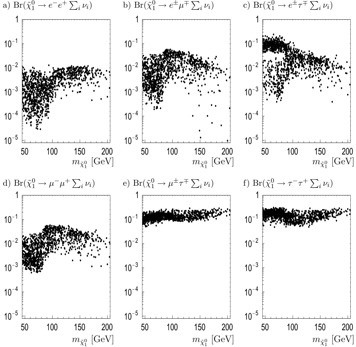
Figure 9: Neutralino branching ratios for the decays into various lepton final states summing over all neutrinos.
