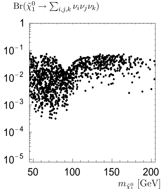
Figure 6: Invisible neutralino branching ratio summing over all neutrinos.
