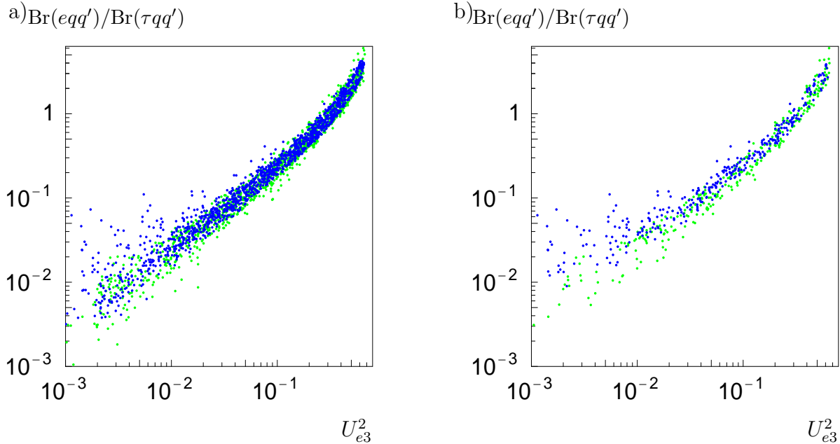
Figure 14: Testing the Chooz angle. In case of the dark (bright) points \mu < (>)0 . In b) we have taken only those points with |\sin 2\theta_b| > 0.1 .
