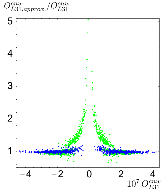
Figure 10: Approximated coupling O_{L31,approx.}^{cnw} using formula eq. (20) divided by the exact calculated coupling as a function of the exact calculated coupling. The bright (dark) points are for \mu > (<)0 .
