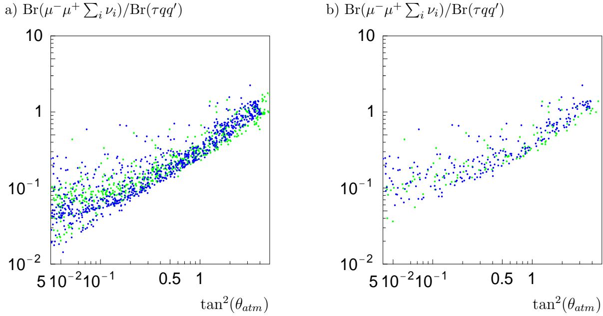
Figure 13: Testing the atmospheric angle. In case of the dark (bright) points \mu < (>)0 . In the second figure we have taken only those points with |\sin 2\theta_b| > 0.1 .
