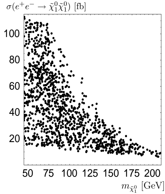
Figure 5: Production cross section for the process \sigma(e^+e^- \rightarrow \tilde{\chi}_1^0\tilde{\chi}_1^0) as a function of m_{\tilde{\chi}_1^0} at a Linear Collider with 1 TeV c.m.s energy. ISR-corrections are included.
