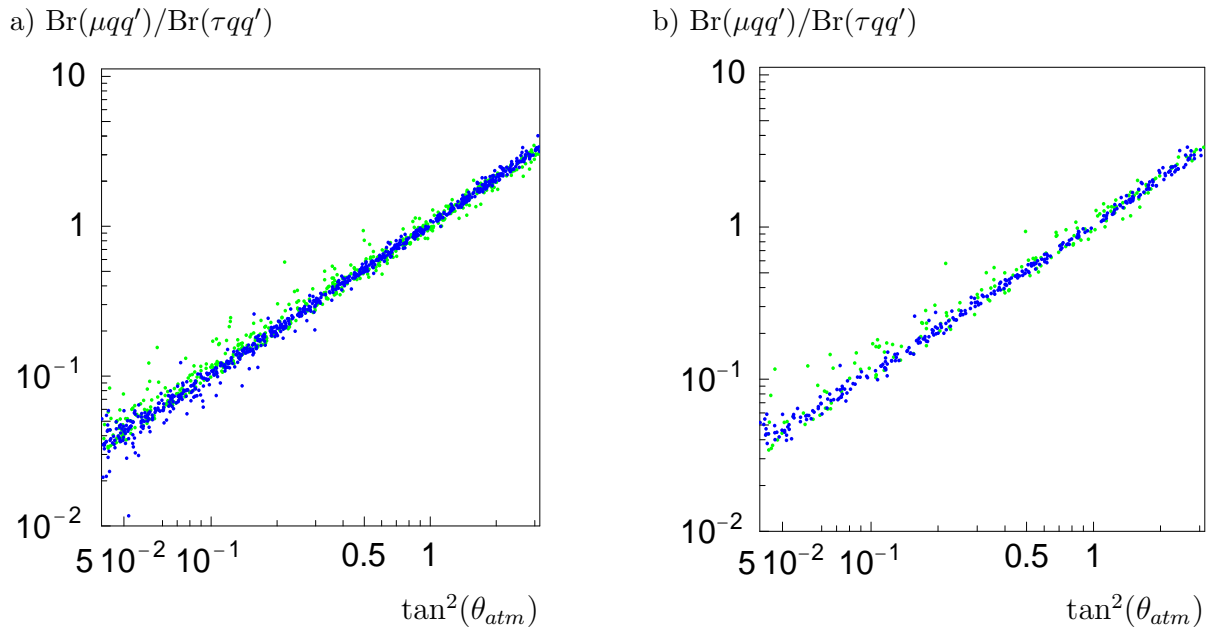
Figure 11: Testing the atmospheric angle. In case of the dark (bright) points \mu < (>)0 . In the second figure we have taken only those points with |\sin 2\theta_b| > 0.1 .
