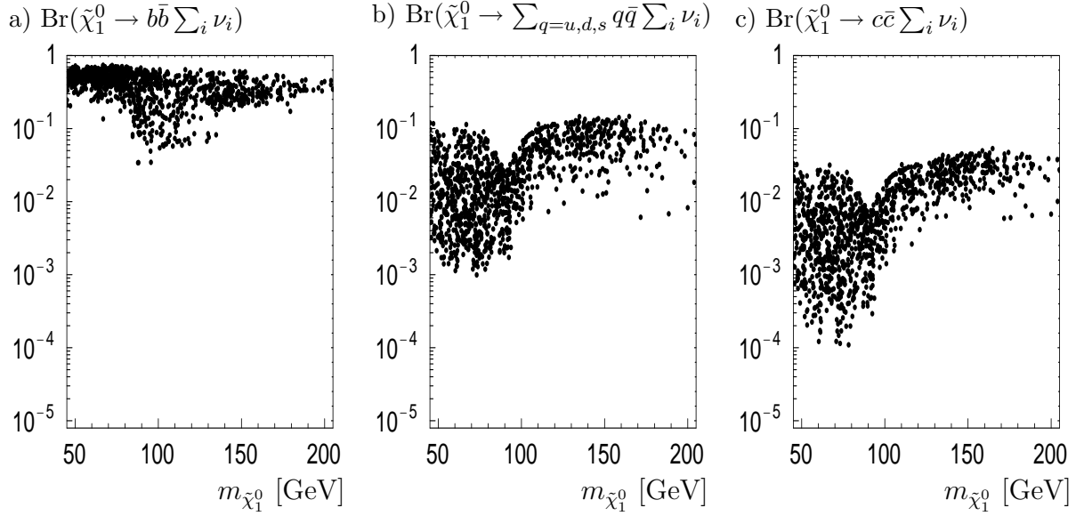
Figure 7: Neutralino branching ratios for the decays into q\bar{q}\nu_i final states summing over all neutrinos.
