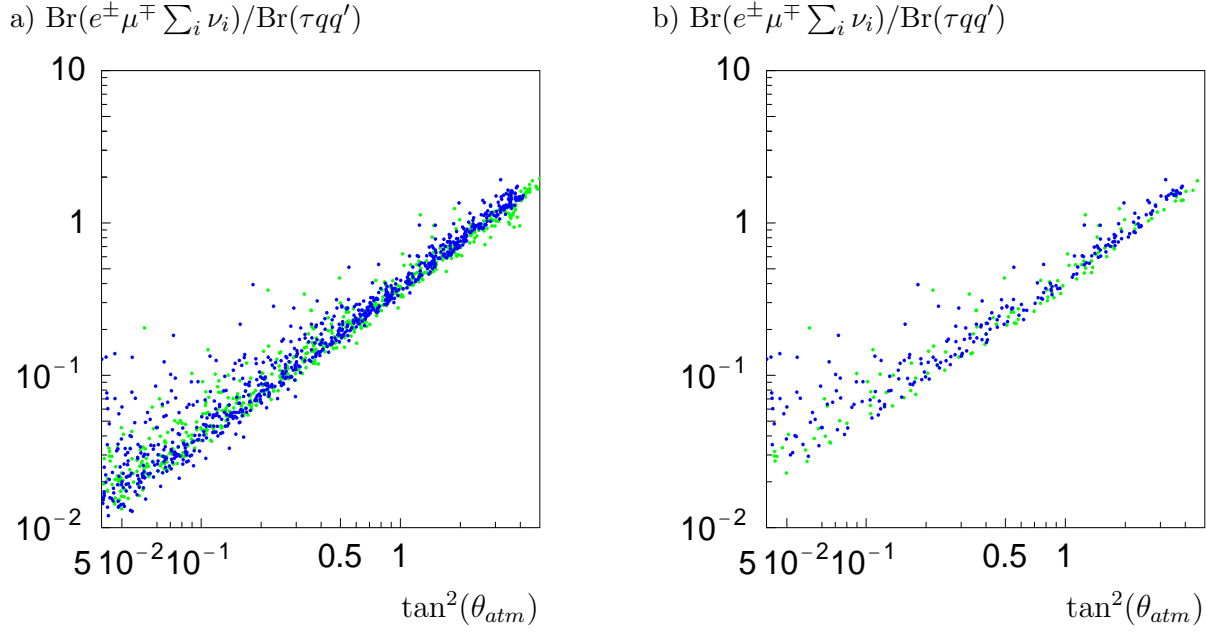
Figure 12: Testing the atmospheric angle. In case of the dark (bright) points \mu < (>)0 . In the second figure we have taken only those points with |\sin 2\theta_b| > 0.1 .
