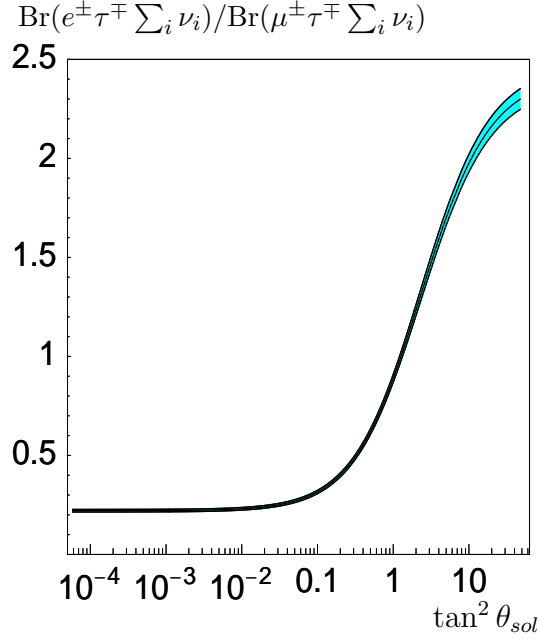
Figure 20: Correlation between \tan^2\theta_{sol} and the ratio \text{Br}(e^\pm\tau^\mp\sum_i\nu_i)/\text{Br}(\mu^\pm\tau^\mp\sum_i\nu_i) for the parameter point specified in the text assuming that 10^5 neutralino decays have been measured. The band corresponds to an 1\text{-}\sigma error.
