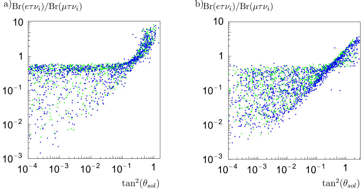
Figure 16: Testing the solar angle. In case of the dark (bright) points \mu < (>)0 . In a) we have taken \epsilon_\mu\Lambda_\mu/(\epsilon_\tau\Lambda_\tau) > 0 . and in b) \epsilon_\mu\Lambda_\mu/(\epsilon_\tau\Lambda_\tau) < 0
