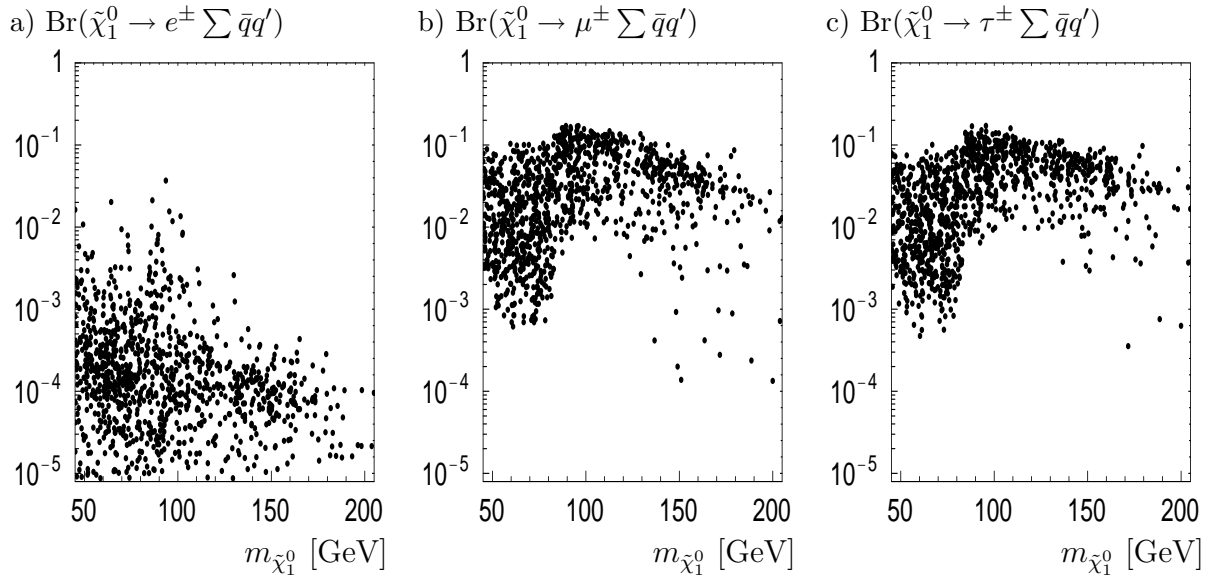
Figure 8: Neutralino branching ratios for the decays into l^\pm q'\bar{q} final states summing over all q'\bar{q} combinations.
