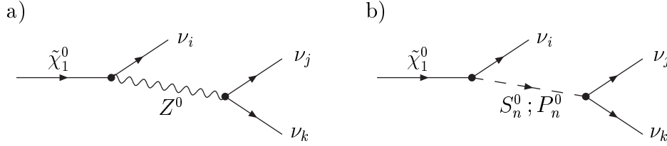
Figure 3: Generic Feynman graphs for invisible neutralino decays.
