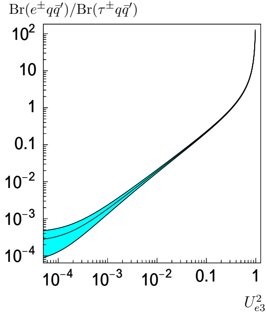
Figure 19: Correlation between U_{e3}^2 and the ratio \text{Br}(e^\pm q\bar{q}')/\text{Br}(\tau^\pm q\bar{q}') for the parameter point specified in the text assuming that 10^5 neutralino decays have been measured. The band corresponds to an 1\text{-}\sigma error.
