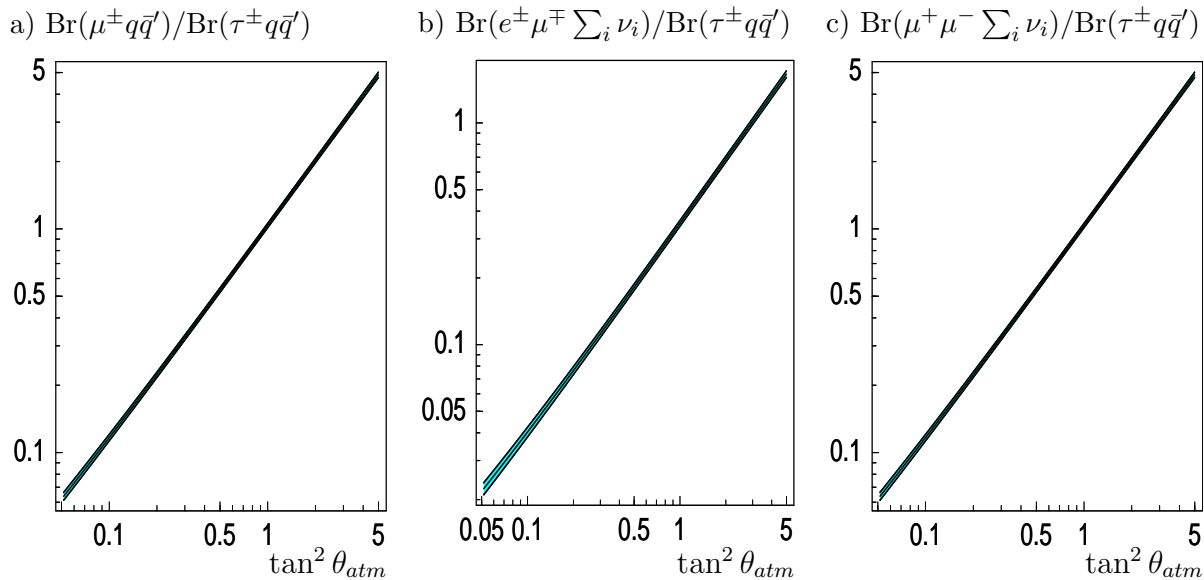
Figure 18: Correlations between \tan^2 \theta_{atm} and ratios of branching ratio for the parameter point specified in the text assuming that 10^5 neutralino decays have been measured. The bands correspond to an 1-\sigma error.
