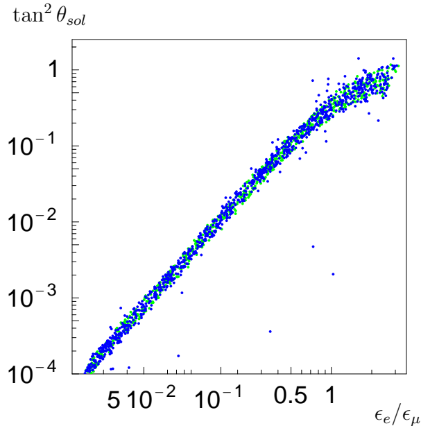
Figure 15: The solar mixing angle as a function of \epsilon_e/\epsilon_\mu .
