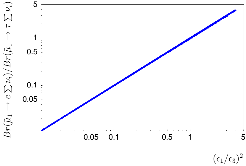
Figure 5: Ratios of branching ratios for scalar tau (top panel) decays versus (\epsilon_1/\epsilon_2)^2 and scalar muon decays (bottom panel) versus (\epsilon_1/\epsilon_3)^2 for Set3.
