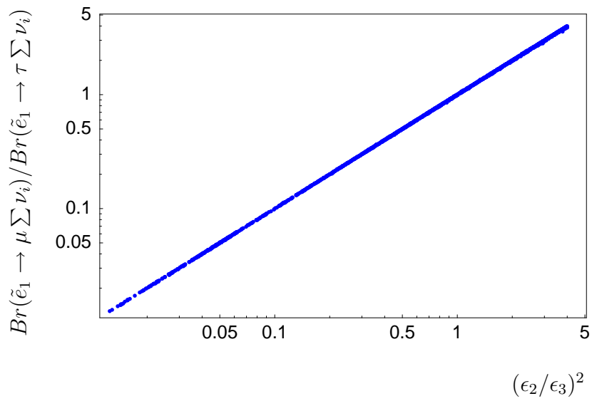
Figure 4: Ratios of branching ratios for scalar electron decays versus (\epsilon_2/\epsilon_3)^2 for Set3.
