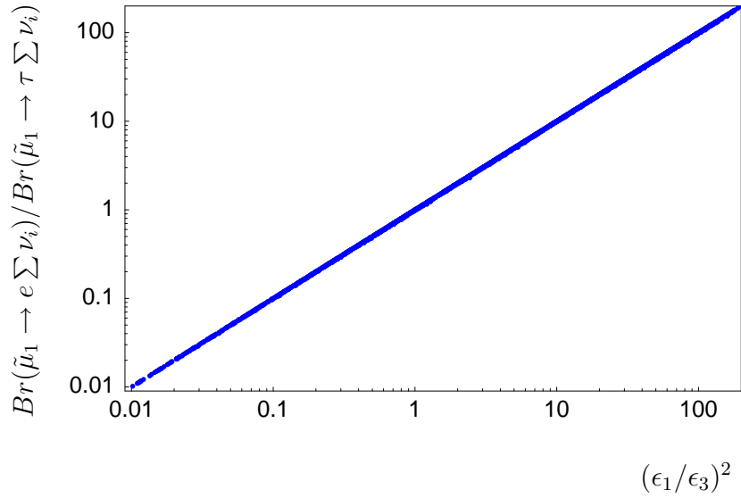
Figure 3: Ratios of branching ratios for scalar tau decays (top panel) versus (\epsilon_1/\epsilon_2)^2 , and scalar muon decays (bottom panel) versus (\epsilon_1/\epsilon_3)^2 for Set2.
