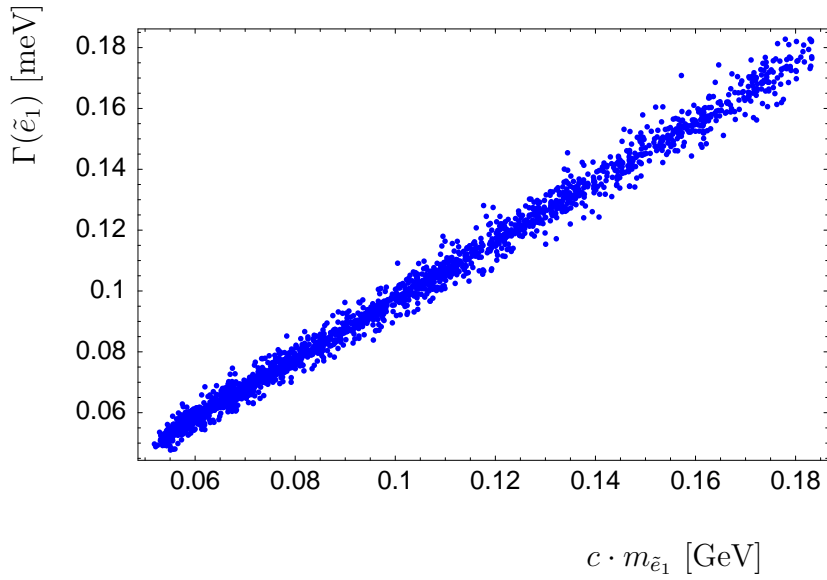
Figure 8: Charged scalar electron total decay widths in [meV], the top panel refers to Set2 while the bottom one is for Set3. The plots are versus c \cdot m_{\tilde{e}_1} , where c = \frac{1}{8\pi}(g')^2 x_1 |\Lambda|^2 .
