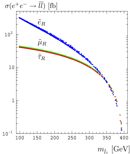
Figure 1: e^+e^- \rightarrow \tilde{l}\tilde{l} production cross section as a function of m_{\tilde{l}} at a Linear Collider with 0.8 TeV c.m.s energy. From top to bottom: \tilde{e} (dark, on colour printers blue), \tilde{\mu} (light shaded, green) and \tilde{\tau} (dark shaded, red).
