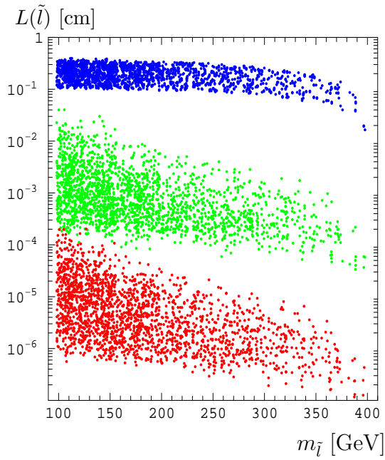
Figure 2: Charged slepton decay length as a function of m_{\tilde{l}} at a linear collider with 0.8 TeV c.m.s. energy. From top to bottom: \tilde{e} (dark, on color printers blue), \tilde{\mu} (light shaded, green) and \tilde{\tau} (dark shaded, red).
