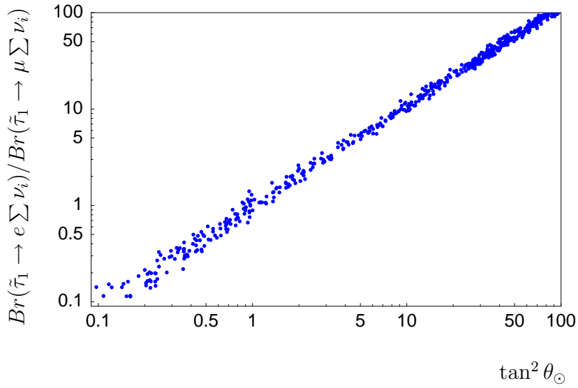
Figure 6: Ratios of branching ratios for scalar tau decays versus \tan^2 \theta_\odot for Set2. The top panel shown all data points, the bottom one refers only to data points with \epsilon_2/\epsilon_3 restricted to the range [0.9, 1.1] .
