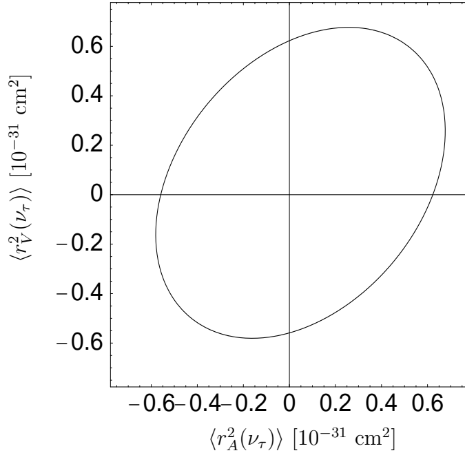
Figure 1: Combined limits on \langle r_V^2(\nu_\tau) \rangle and \langle r_A^2(\nu_\tau) \rangle for Dirac tau neutrinos derived from LEP-2 data. The plot shows the \chi^2_{\min} + 2.71 contour, corresponding to 90 % c.l.
