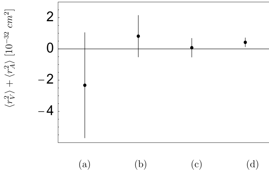
Figure 2: 90 % c.l. limits on (\langle r_V^2 \rangle + \langle r_A^2 \rangle) for the muon neutrino derived from (a) E734 at BNL [28], (b) CHARM II [27], (c) CCFR experiment [60] and (d) from the NuTeV result [56].
