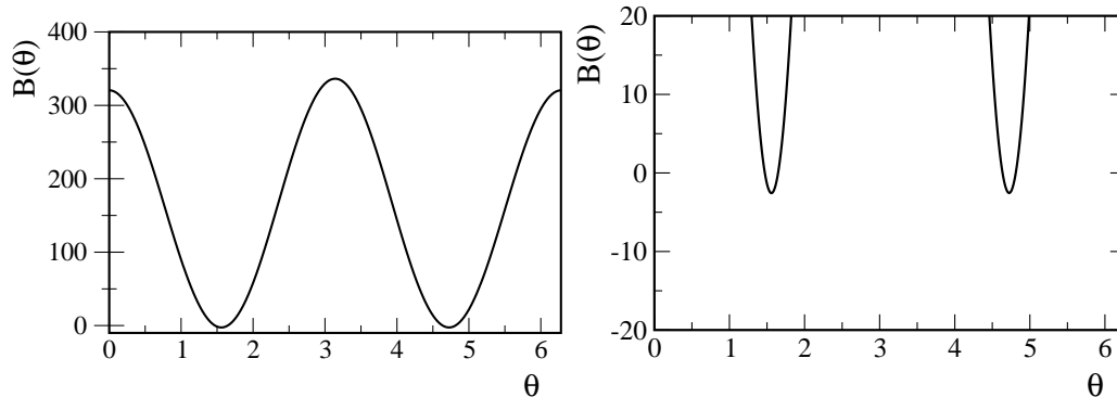
FIG. 1: B(\theta) as a function of \theta for an example where B(\theta_{min}) < 0 but B(0) > 0 . The right panel is an enlarged view of the left one close to the zeros of B(\theta) .
