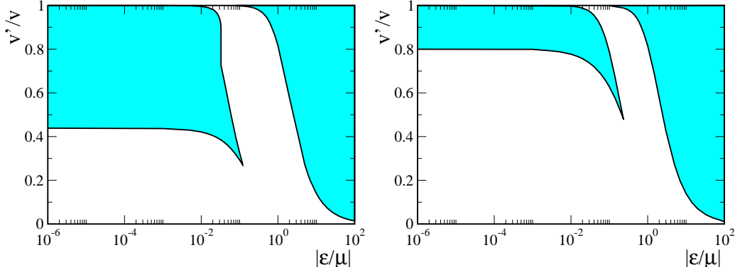
FIG. 2: Range of RMSSM parameters where nonzero charged vev's for the Higgs and slepton fields are favoured over the realistic minimum for two examples of \tan\beta , left \tan\beta = 1.05 , right \tan\beta = 1.2 . Here we fix for convenience B = B' = \mu = 100 GeV. For a discussion see text.
