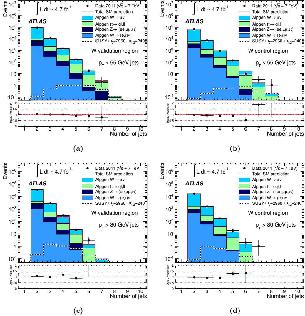
Figure 3. Jet multiplicity distributions for the W^\pm + jets validation regions (left) and control regions (right) before any jet multiplicity requirements, and for a jet p_T threshold of 55 GeV (top) and 80 GeV (bottom).
