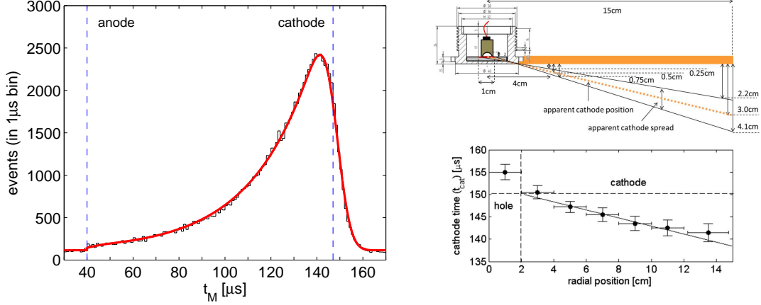
Figure 9. Sketch of the procedure used for determining the TPC drift region under \gamma irradiation at E_{drift}/P = 145.5 V/cm/bar, P = 1 bar. Left: time distribution and fit to the function introduced in the text (red line). Right-up: approximate sketch of the geometry in the source region. Right-down: the apparent position of the cathode for different slices in the radial position of the energy deposit ( r_{evt} ) as obtained from the left fit. The estimate of the cathode position ( t_{cat} = 150 \mu\text{s} ) from this differential analysis differs by about 2% with respect to a global fit ( t_{cat} = 147 \mu\text{s} ).
