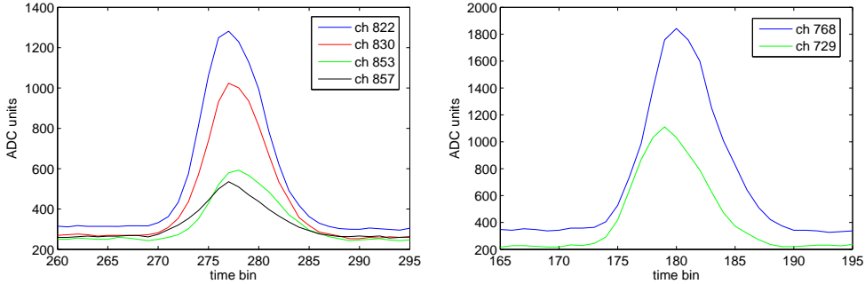
Figure 7. Events obtained from a high purity \gamma -ray sample in a narrow energy window 25\text{ keV} < \epsilon_{evt} < 35\text{ keV} after x - y and z -fiducialization, and after performing a width – time correlation cut (see the text for details).
