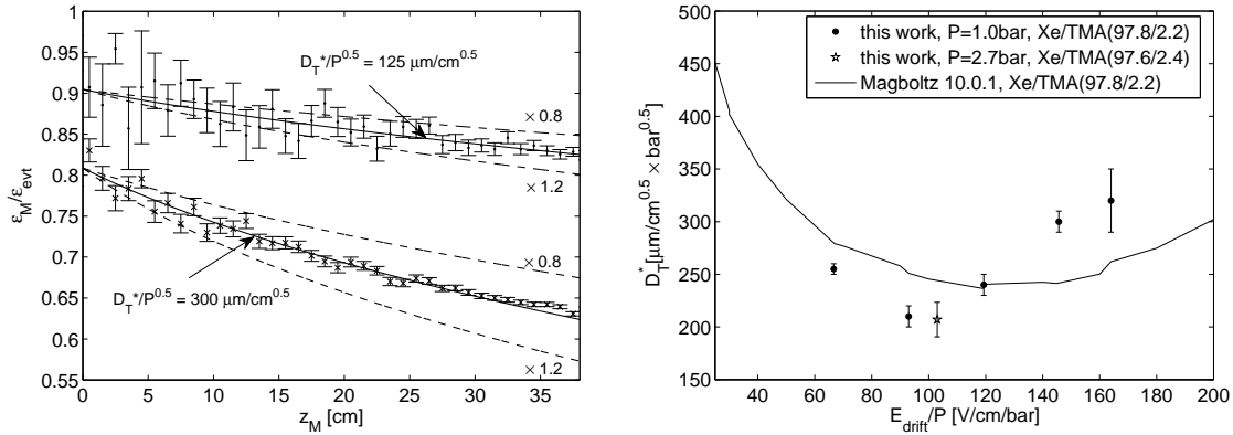
Figure 13. Left: behaviour of the highest charge fraction contained in a single pixel \varepsilon_M/\varepsilon_{evt} as a function of the z -position of the deposit for E_{drift}/P = 145.5 V/cm/bar at P = 1 bar (crosses) and E_{drift}/P = 103.6 V/cm/bar at P = 2.7 bar (points). The transverse diffusion coefficients extracted from the fit proposed in the text are indicated together with the trends for 20% variations around it, to illustrate the sensitivity of the method. Right: transverse diffusion coefficient obtained from this analysis including statistical uncertainties only. Systematic effects related to the naive treatment of the initial ionization cloud have not been evaluated.
