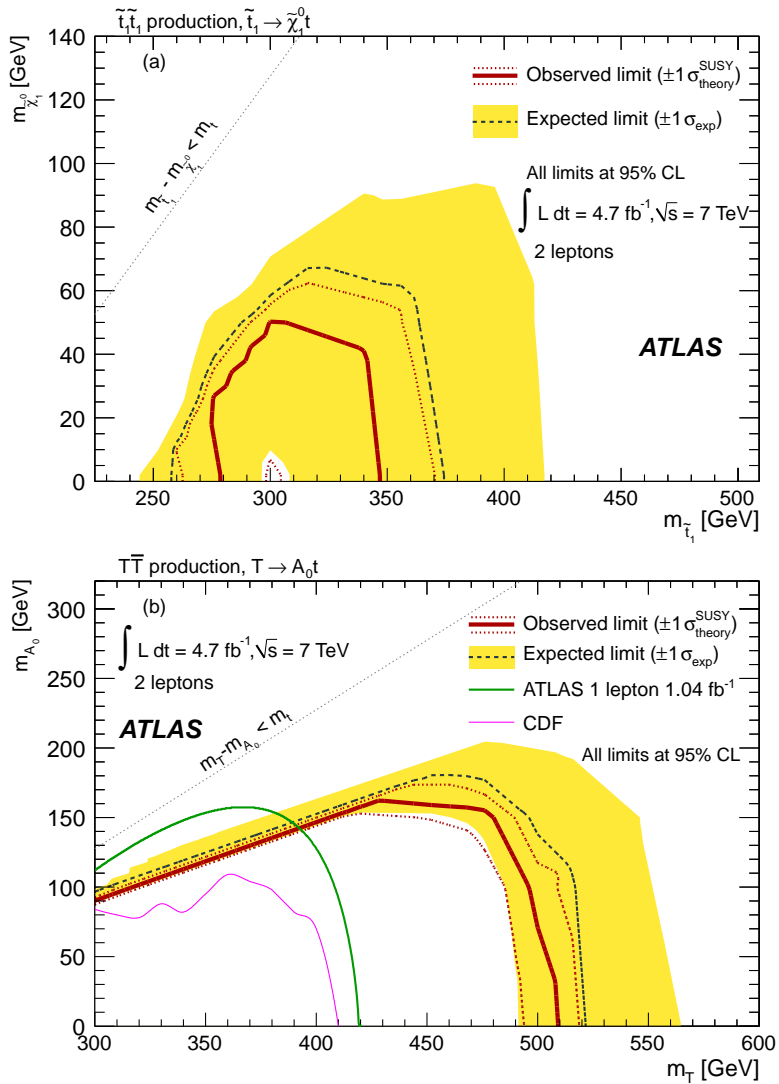
Figure 2. Expected and observed 95% CL limits (a) in the \tilde{t}_1 \rightarrow t \tilde{\chi}_1^0 model as a function of the scalar top and neutralino masses, and (b) in the T \rightarrow t A_0 model as a function of the spin-1/2 top-quark partner T and A_0 masses. The dashed line and the shaded band are the expected limit and its \pm 1\sigma uncertainty, respectively. The thick solid line is the observed limit for the central value of the signal cross section. The expected and observed limits do not include the effect of the theoretical uncertainties on the signal cross section. The dotted lines show the effect on the observed limit of varying the signal cross section by \pm 1\sigma of the theoretical uncertainty. The curve labelled “ATLAS 1 lepton 1.04 fb -1 ” is the previous ATLAS limit from ref. [25] using the one lepton channel while the curve labelled “CDF” is from ref. [24].
