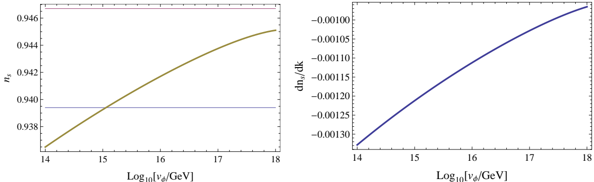
Figure 2: The spectral index n_s and its running as a function of v_\phi in the standard CW inflation. Two horizontal lines in the left panel show 2\sigma and 3\sigma lower bounds measured by Planck, respectively.
