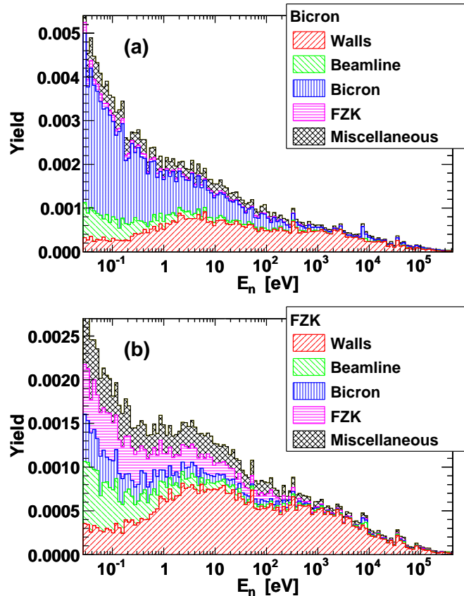
Figure 10: (Color online) Stacked contributions to the neutron background yield of ^{13}\text{C} for both \text{C}_6\text{D}_6 detectors – Bicorn (a) and FZK (b) – coming from the different sets of experimental components. Note that absolute scales for two detectors differ by a factor of 2.
