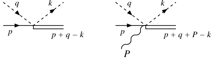
FIG. 10: S -wave kaon-nucleon vertex and the corresponding \phi contact coupling.
