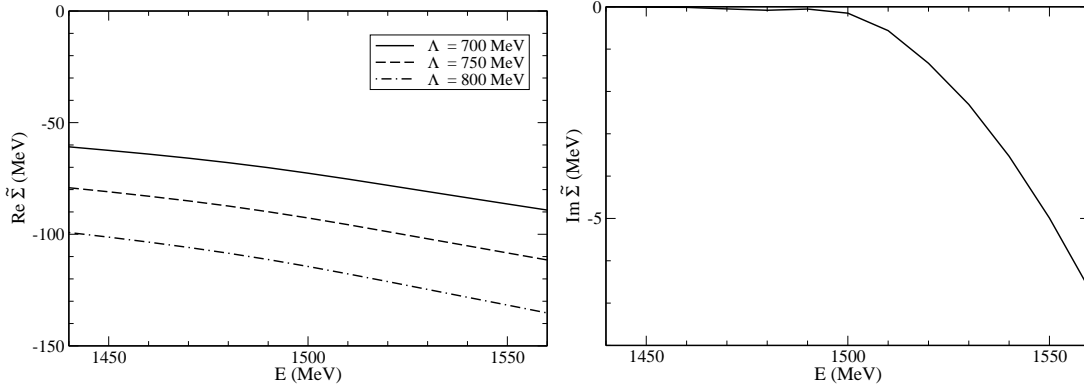
Figure 2. \Theta^+ selfenergy in the medium for \rho = \rho_0 .
