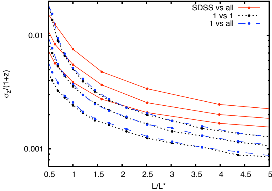
Figure 13. Photo- z error as a function of luminosity. Solid lines: Redshifted SDSS DR6 galaxies are fitted with our five templates. Dashed lines: Same results when galaxies are generated with template 1, and fitted with five templates. Dotted lines: Same results for galaxies generated with template 1 and fitted with the same template. The redshift error is the 68 percentile of the averaged distribution over each redshift interval of width \Delta z = 0.1 , centered at z = 0.65 , 0.75 and 0.85 (errors increase with redshift).
