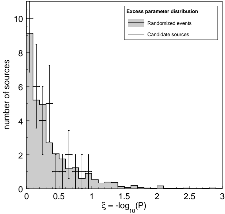
FIG. 7: Excess parameter ( \xi ) distribution from the search for neutrinos from pre-selected objects. The results of each individual observation (data points) are compared to the expected distribution from 1000 simulated equivalent experiments with randomized right ascension (filled histogram).
