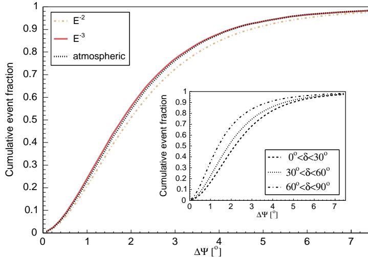
FIG. 2: Cumulative point spread function for the events passing the selection, for different simulated energy spectra. The inset graph shows the dependence on declination, for a spectral index \gamma=2 . \Delta\Psi is the space angle difference between the true and the reconstructed direction of simulated events.
