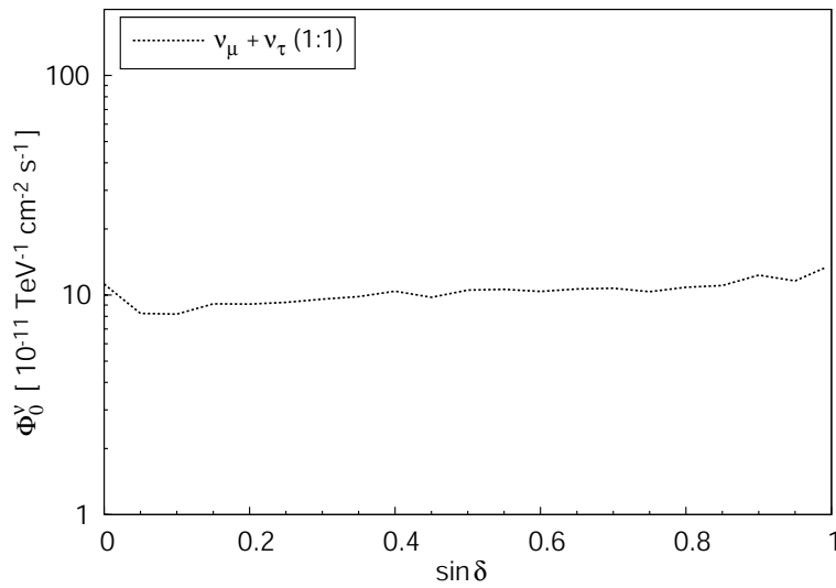
FIG. 5: Sensitivity to point sources of neutrinos as a function of declination, for an integrated exposure of 1001 days and for a \gamma=2 source spectrum. The sum of muon and tau neutrinos fluxes is considered assuming \Phi_{\nu_\mu + \bar{\nu}_\mu} / \Phi_{\nu_\tau + \bar{\nu}_\tau} = 1
