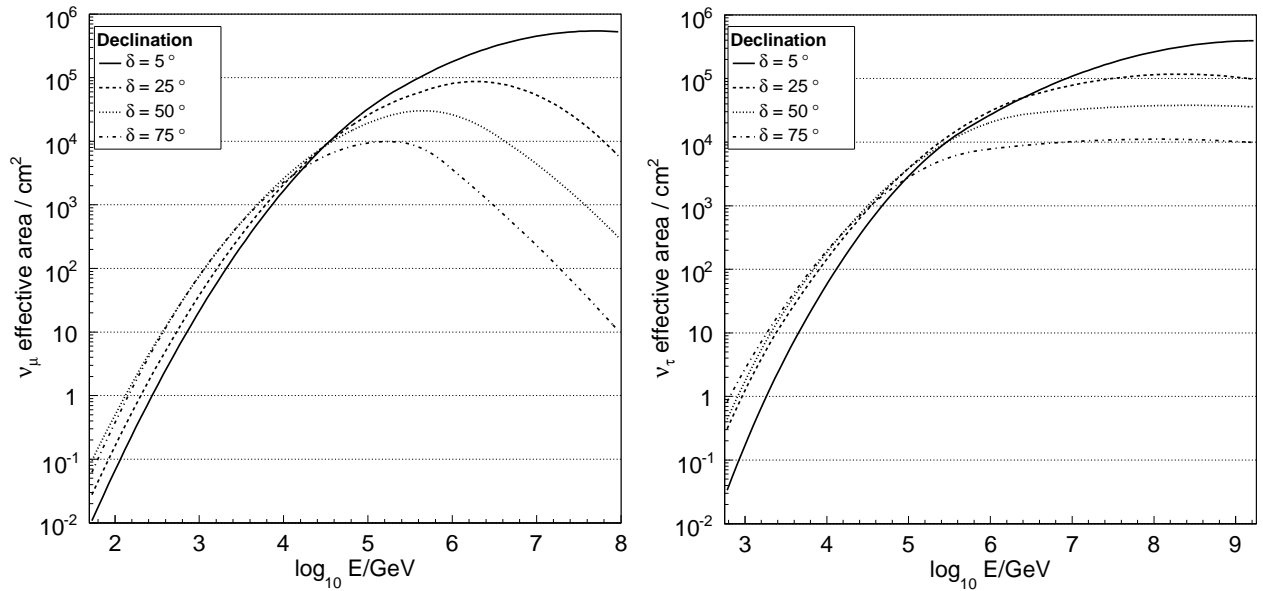
FIG. 4: Neutrino effective area as a function of the neutrino energy for different declinations for muon neutrinos (left) and tau neutrinos (right) respectively. The decrease observed at high energies on the left is due to neutrino absorption in the earth.
