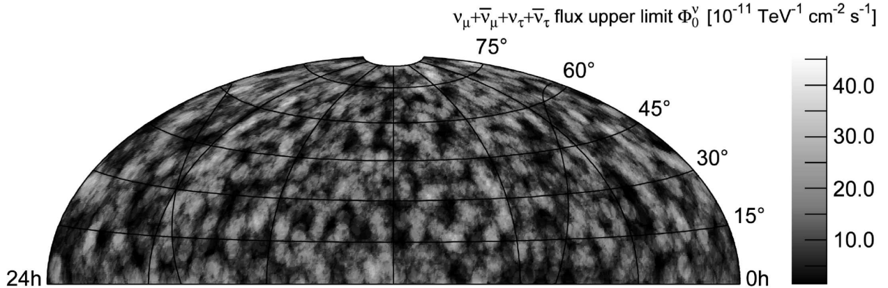
FIG. 8: Map of the 90% CL upper limits to the muon and tau neutrino flux from the survey of the northern sky, for a spectral index \gamma=2 . Limits are given on the normalization factor \Phi^0 to the flux \frac{d\Phi}{dE} = \Phi^0 \cdot \left(\frac{E}{1\text{TeV}}\right)^{-\gamma} .
