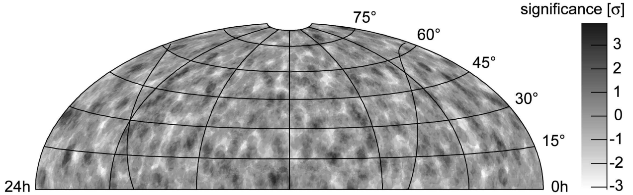
FIG. 6: Sky map of the significance obtained by scanning of the northern sky to search for event clusters. The significance is positive for excesses and negative for deficits of events compared to the expected background.
