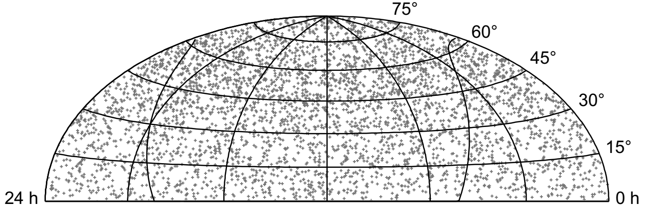
FIG. 3: Sky-plot of the selected 4282 upward going neutrino candidate events. Horizontal coordinates are given as right ascension and vertical coordinates as declination. The black line marks the location of the galactic plane.
