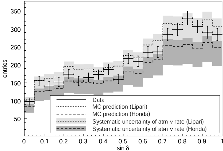
FIG. 1: Declination angle distribution of the final event selection compared to the expectation from Monte Carlo simulation of atmospheric neutrinos, including the systematic error band (see Section V). The two extremes [25, 26] among different predictions are shown. Error bars on the data point are statistical.
