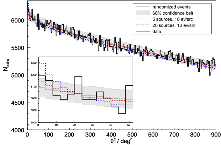
FIG. 9: Distribution of the separation angle between event pairs for the experimental data and for two samples consisting of the original data plus signal events following the point spread function of the detector (5 and 20 sources respectively, each contributing 10 neutrinos on average). The distribution expected for a pure atmospheric sample is also shown (randomized events) with a 1\sigma confidence belt.
