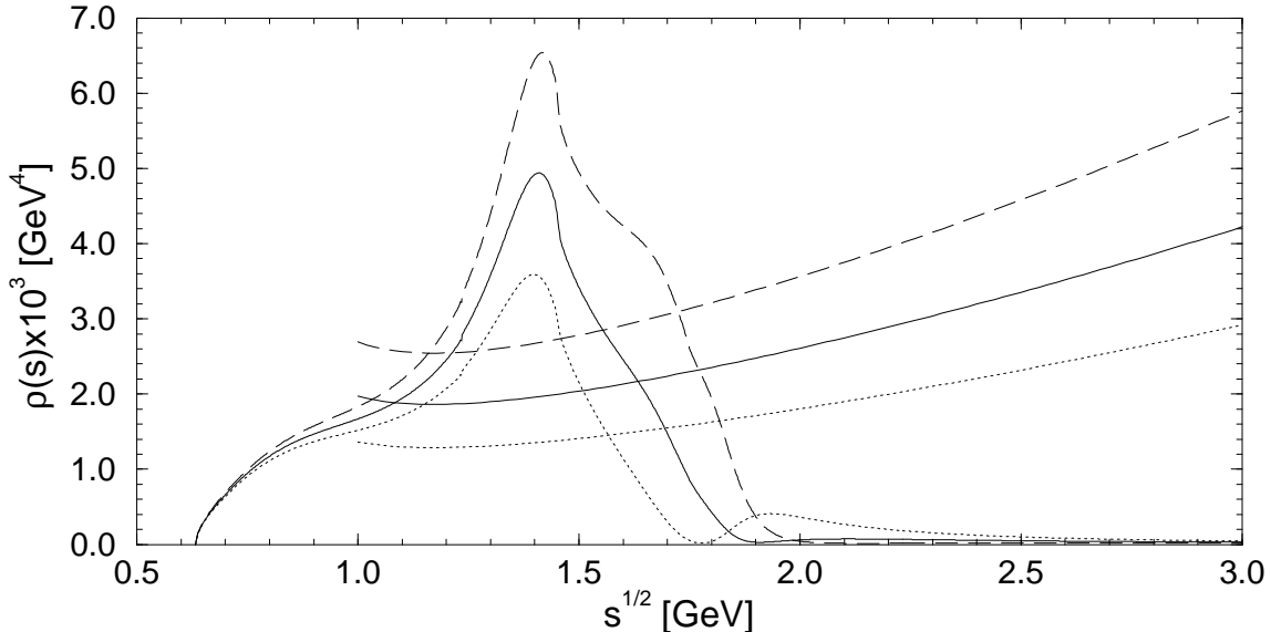
Figure 2: The theoretical as well as phenomenological spectral functions used in our m_s determination. Solid lines: central spectral functions; long-dashed lines: \rho_{ph}(s) for (6.10K4) with F_{K\pi}(\Delta_{K\pi}) = 1.23 and \rho_{th}(s) for m_s = 115 MeV; dotted lines: \rho_{ph}(s) for (6.10K3) with F_{K\pi}(\Delta_{K\pi}) = 1.21 and \rho_{th}(s) for m_s = 83 MeV.
