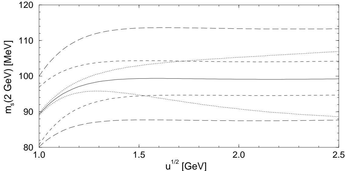
Figure 1: The strange mass m_s(2 \text{ GeV}) as a function of \sqrt{u} . Solid line: central parameters; long-dashed lines: (6.10K4) with F_{K\pi}(\Delta_{K\pi}) = 1.23 (upper line), (6.10K3) with F_{K\pi}(\Delta_{K\pi}) = 1.21 (lower line); dashed lines: \alpha_s(M_Z) = 0.1205 (lower line), \alpha_s(M_Z) = 0.1165 (upper line); dotted lines: s_0 = 4.2 \text{ GeV}^2 (upper line), s_0 = 5.8 \text{ GeV}^2 (lower line).
