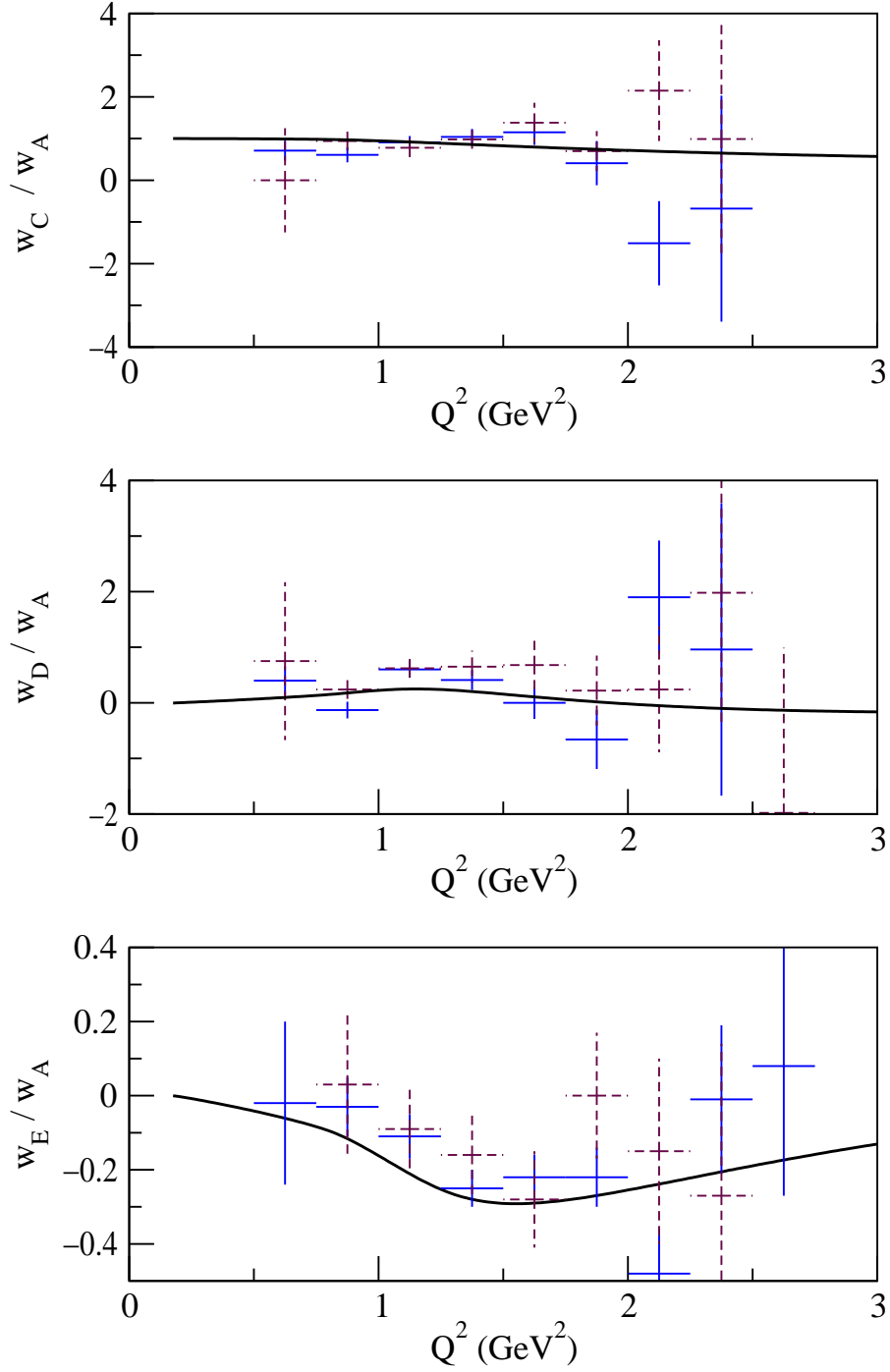
Figure 7: Experimental data for w_C , w_D and w_E integrated structure functions, normalized to w_A . Solid (dashed) bars correspond to the values quoted by CLEO-II (OPAL) [8].
