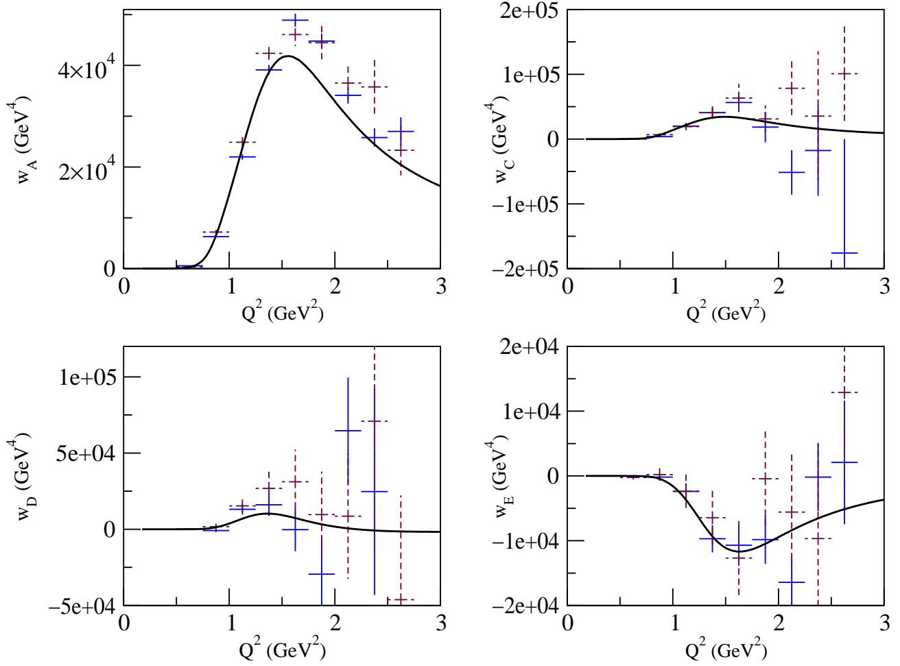
Figure 5: Theoretical values for the w_A , w_C , w_D and w_E integrated structure functions in comparison with the experimental data from CLEO-II (solid) and OPAL (dashed) [8]. All of them have been normalized to their respective branching ratios.
