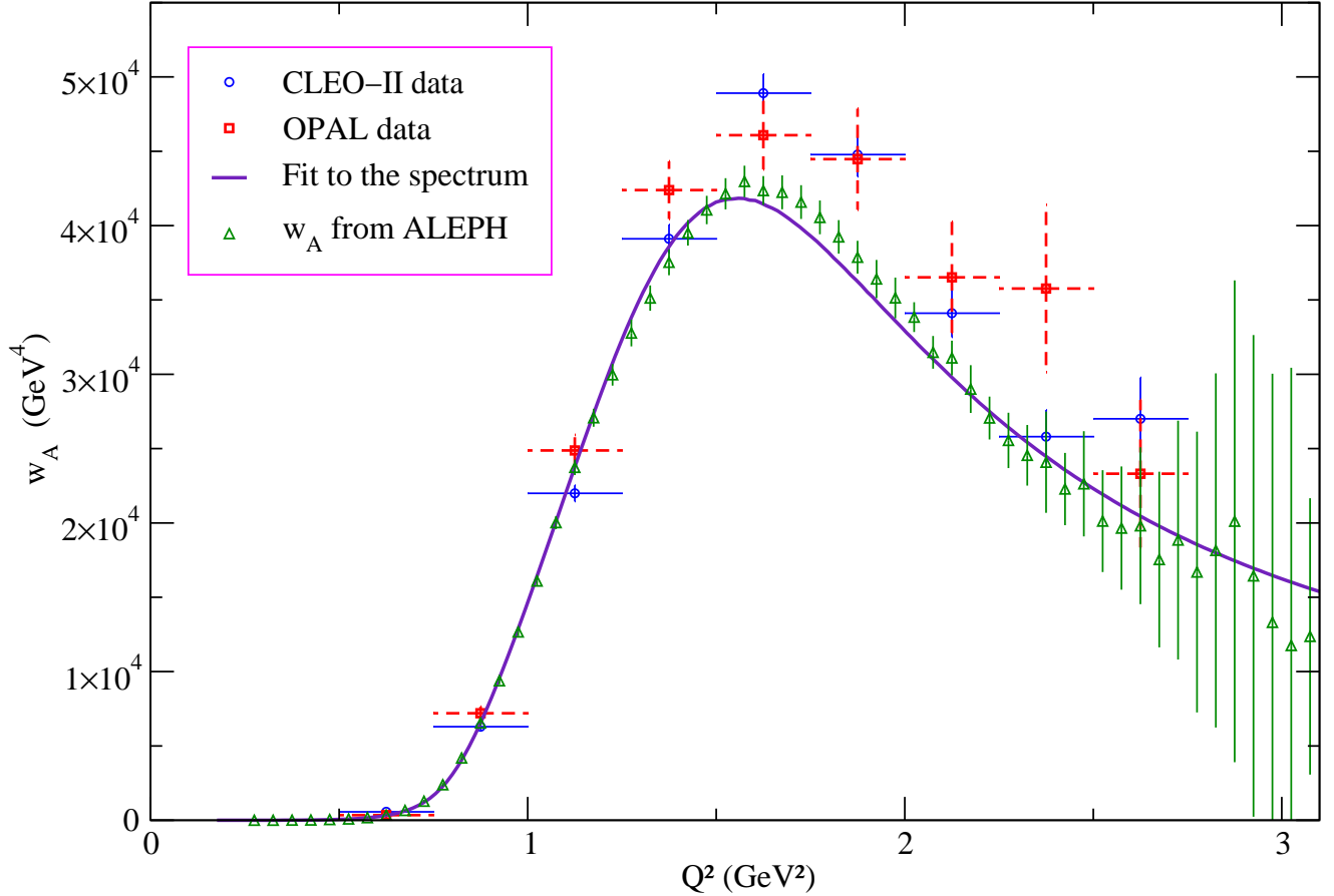
Figure 6: Comparison between the experimental data for w_A , from \tau^- \rightarrow \pi^- \pi^0 \pi^0 \nu_\tau , quoted by CLEO-II and OPAL [8] and the values arising from ALEPH measurements of \tau^- \rightarrow \pi^+ \pi^- \pi^- \nu_\tau spectral functions [6]. The solid line is obtained from our four-parameter fit of the spectrum (see text).
