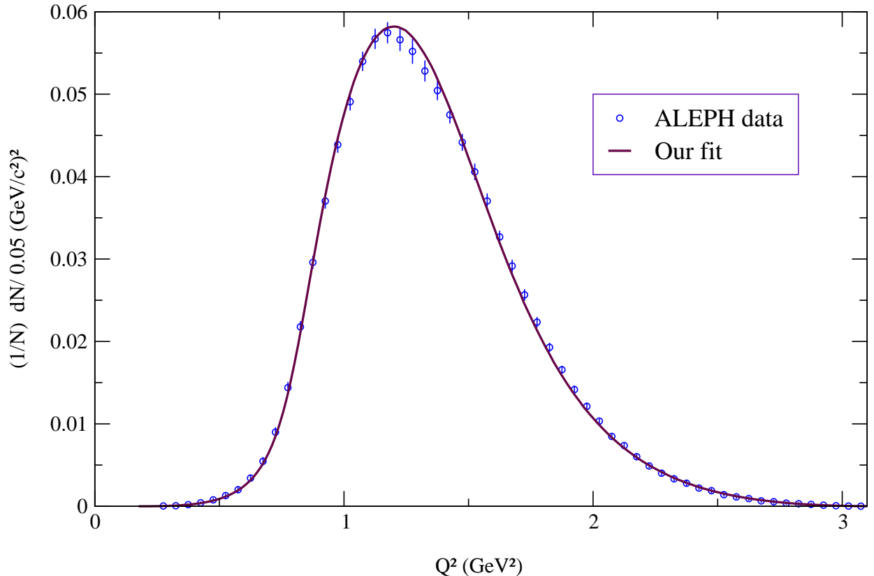
Figure 3: Fit to the ALEPH data for the normalized \tau^- \rightarrow \pi^+\pi^-\pi^-\nu_\tau spectral function.
