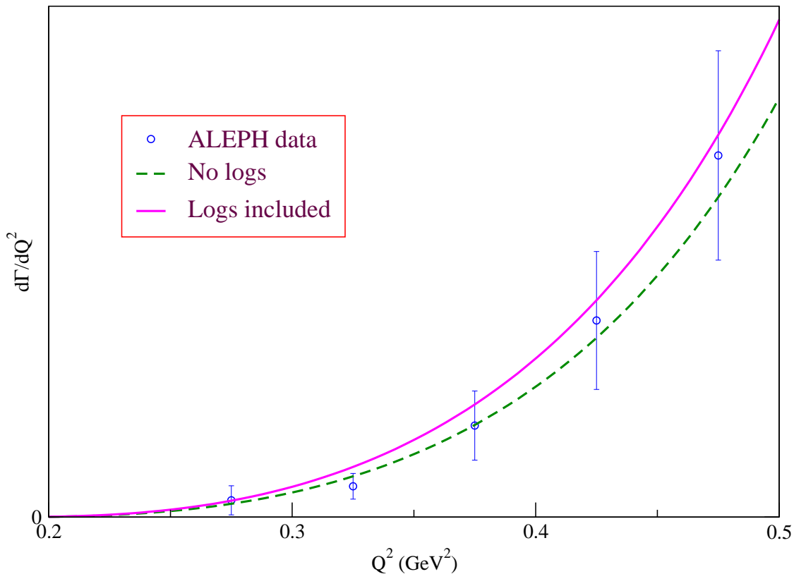
Figure 4: Theoretical curves for \tau^- \rightarrow \pi^+\pi^-\pi^-\nu_\tau spectrum at Q^2 \ll M_V^2 , with and without the inclusion of chiral logs, vs. ALEPH data in the low Q^2 region [6].
