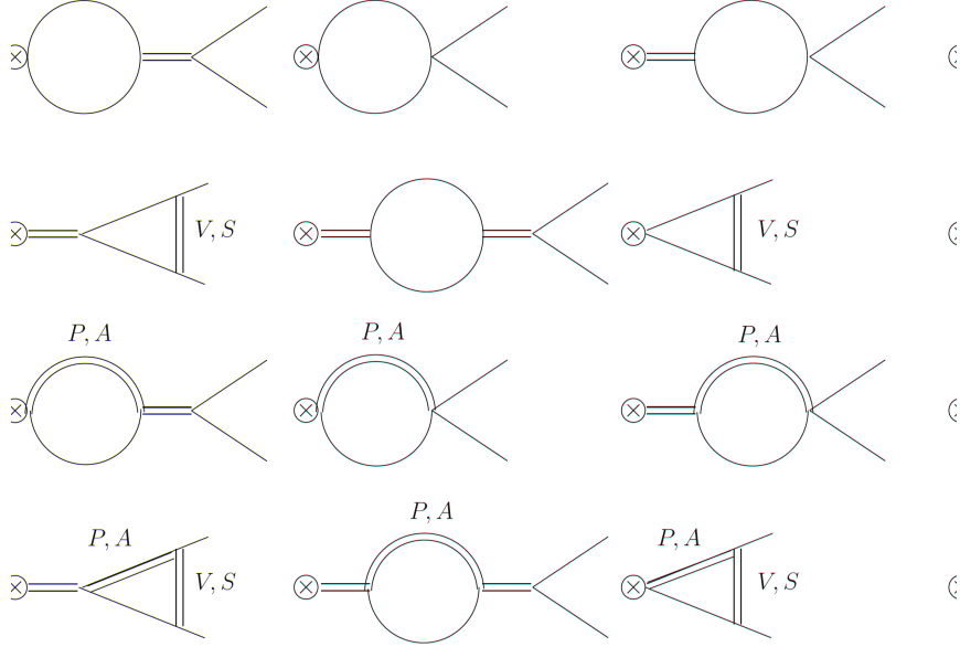
Figure 2: One-loop contributions to the vector form factor of the pion with absorptive cut. A single line stands for a pseudo-Goldstone boson while a double line indicates a resonance.
