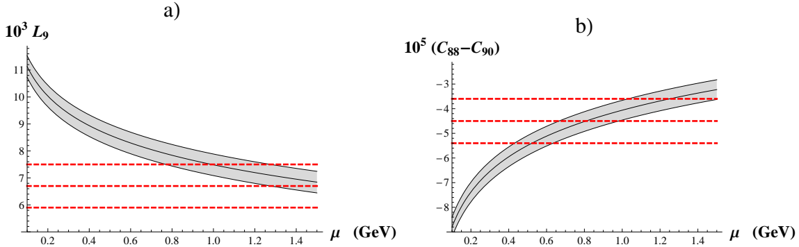
Figure 3: The R \chi T predictions (solid gray band) for the \chi PT \mathcal{O}(p^4) low-energy constant L_9(\mu) (a) and the \mathcal{O}(p^6) combination C_{88}(\mu) - C_{90}(\mu) (b) are compared to their large- N_C estimates (red dashed) for different values of the renormalization scale \mu . The error of the large- N_C estimate is given by the naive saturation scale uncertainty from eq. (4.9).
