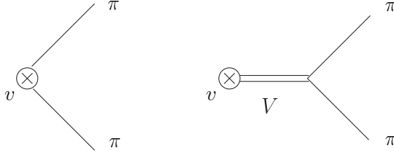
Figure 1: Tree-level contributions to the vector form factor of the pion. A single line stands for a pseudo-Goldstone boson while a double line indicates a resonance.
