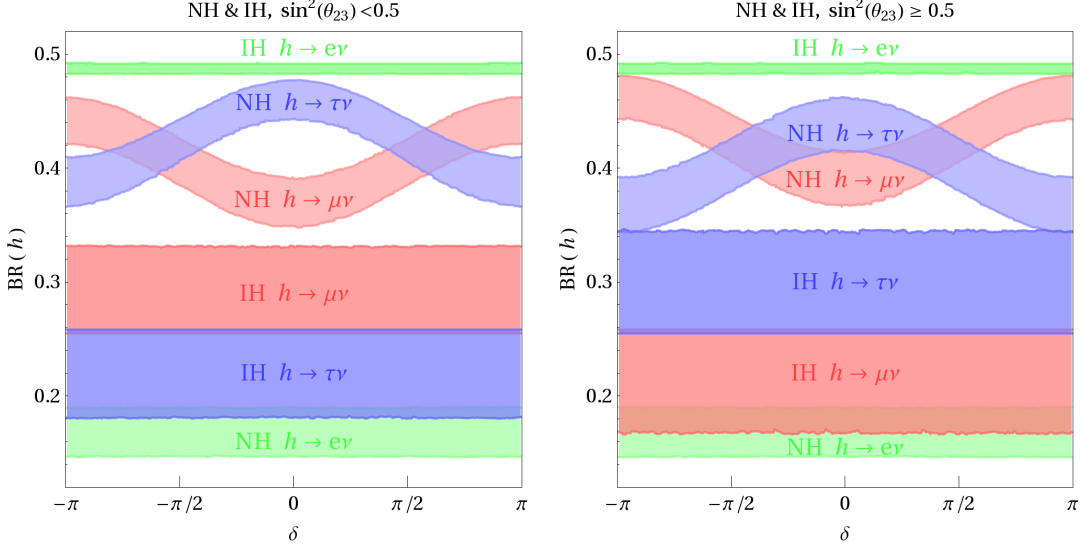
Figure 8: Branching ratios of the charged singlet h to e\nu , \mu\nu , \tau\nu splitting the two currently allowed octants of \theta_{23} , \theta_{23} < 45^\circ ( \theta_{23} > 45^\circ ) left (right). One can see the dependence on \delta for the NH spectrum in the \mu\nu and \tau\nu channels. The most significant change between octants is the interchange of the \mu\nu and \tau\nu for the IH case. The bands are 95% C.L. regions.
