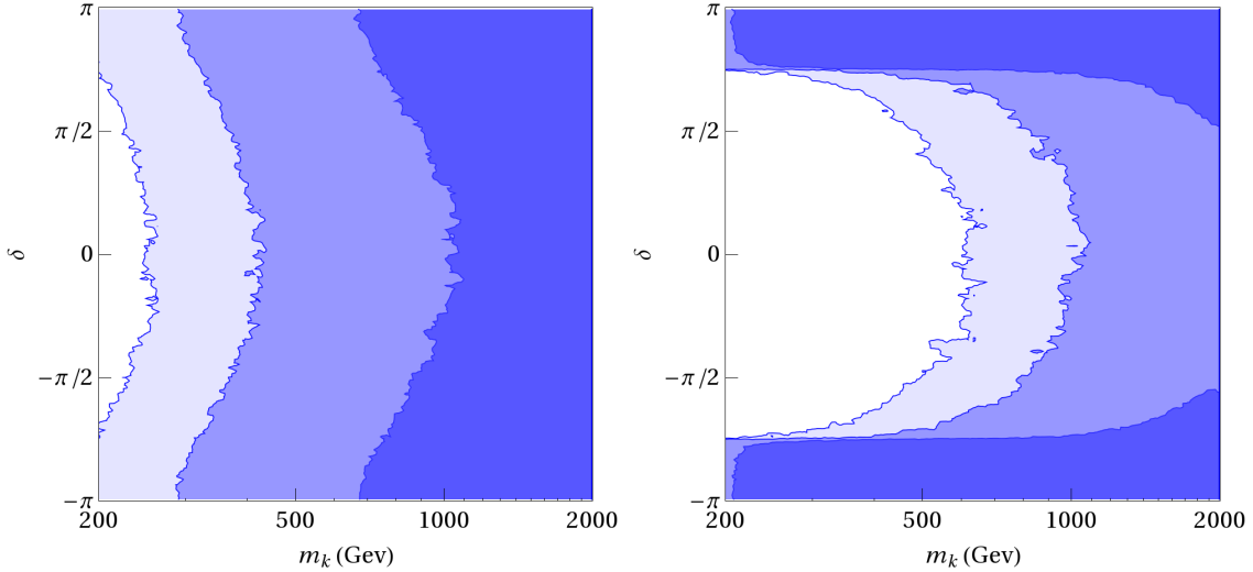
Figure 7: \delta vs m_k in NH (left) and IH (right).
