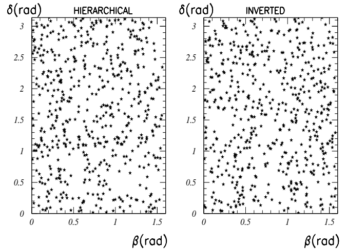
FIG. 1: A random selection of points where the baryon asymmetry is large enough, for some choice of the unmeasurable parameters of the seesaw. The light neutrino masses are taken non-degenerate, and the Majorana phase of the smallest one can be neglected. The “Dirac” phase \delta is defined such that U_{e3} = \sin \theta_{13} e^{-i\delta} , and \beta is the majorana phase of m_2 = |m_2| e^{2i\beta} . The baryon asymmetry arises in the decay of N_1 of mass M_1 = 10^{10} GeV.
