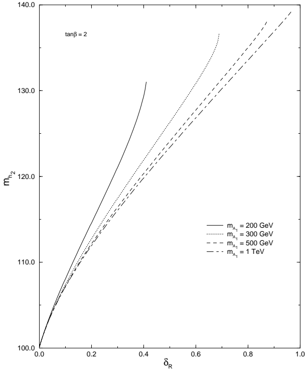
Figure 3: m_{h_1} and m_{h_2} as a function of \delta_R for m_{A_1} = 200, 300, 500, 1000 GeV and m_{A_2} = 100 GeV. The input parameters for the loop contributions to the difference between the CP-even and CP-odd mass matrices are m_Q = 500 GeV, m_U = m_D = 300 GeV, A = 200 GeV, and \mu_I = (200, 0) . In the plots on the left, \tan \beta = 2 ; \tan \beta = 10 for the plots on the right.
