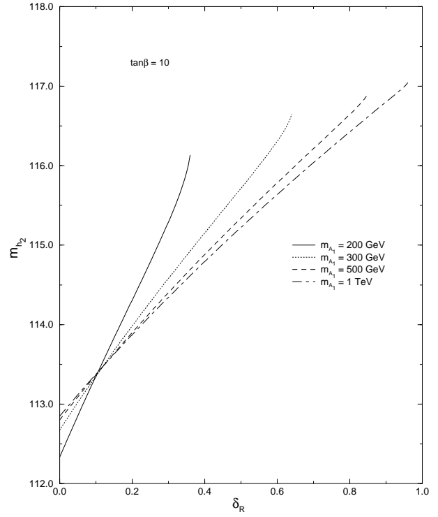
Figure 3: m_{h_1} and m_{h_2} as a function of \delta_R for m_{A_1} = 200, 300, 500, 1000 GeV and m_{A_2} = 100 GeV. The input parameters for the loop contributions to the difference between the CP-even and CP-odd mass matrices are m_Q = 500 GeV, m_U = m_D = 300 GeV, A = 200 GeV, and \mu_I = (200, 0) . In the plots on the left, \tan \beta = 2 ; \tan \beta = 10 for the plots on the right.
