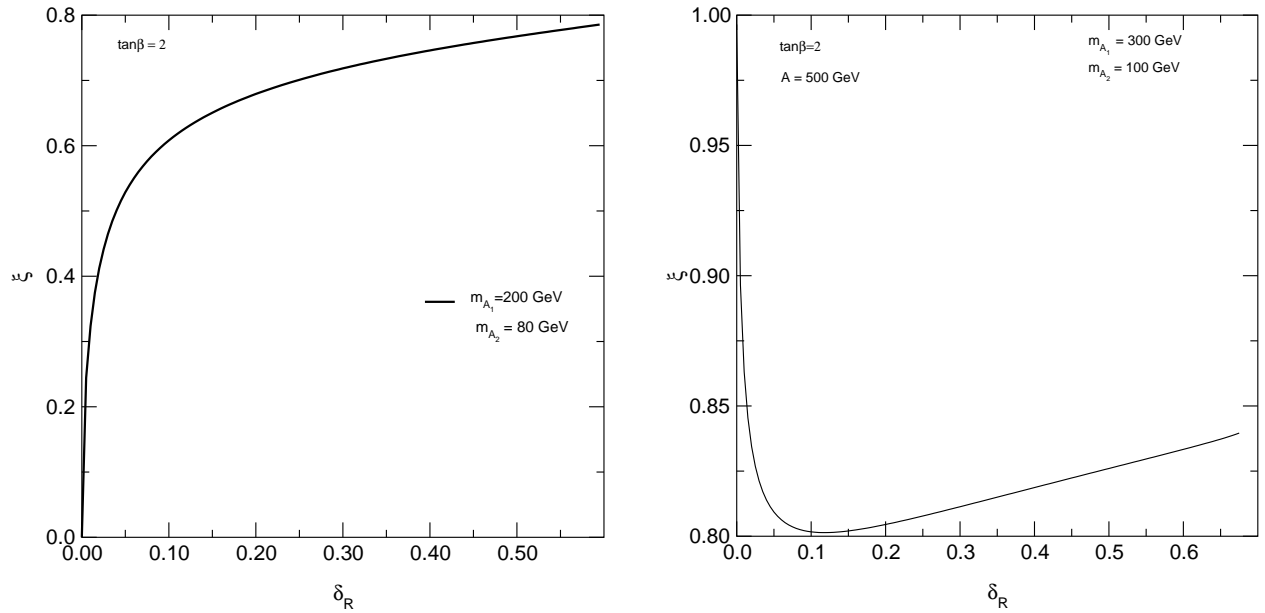
Figure 6: The ratio \xi as a function of \delta_R , where \xi = g_{ZZh}/g_{ZZh}^{SM} is the ratio of the ZZh vertex its value in the SM. When the lightest CP-even scalar h_1 corresponds to the sneutrino in the \delta_R \rightarrow 0 limit, \xi can be small and goes to zero with \delta_R . If m_{A_2} (which becomes m_{\tilde{\nu}} when \delta_R = 0 ) is large, \xi is near its MSSM value.
