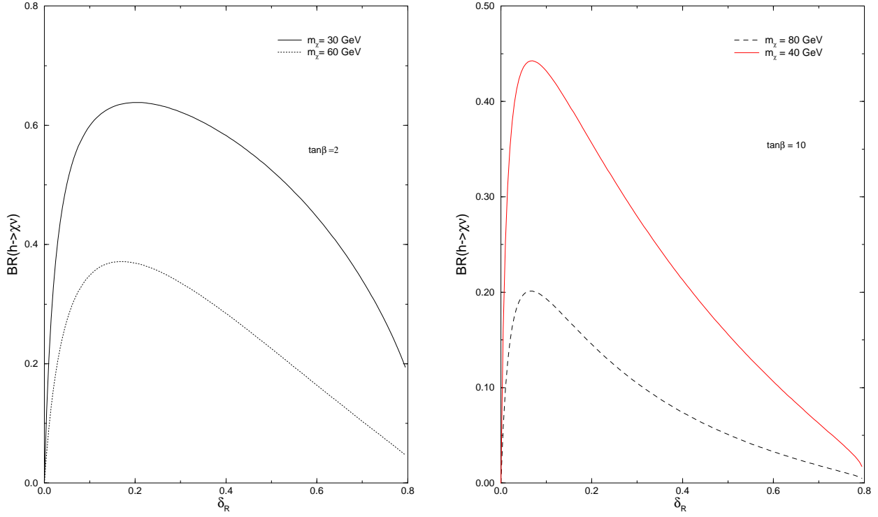
Figure 5: The branching ratio for h_1 \rightarrow \chi^0 \nu as a function of \delta_R , for different values of m_\chi and \tan\beta . We take m_{A_1} = 500 GeV, m_{A_2} = 120 GeV, and the input parameters for the loops contributing to the CP-even—CP-odd Higgs mass difference are A = 0 , \mu_I = (200, 0) , m_Q = 500 GeV, m_U = m_D = 300 GeV. We take the total decay rate to be \Gamma_{tot} = \Gamma(h \rightarrow b\bar{b}) + \Gamma(h \rightarrow \chi^0 \nu) .
