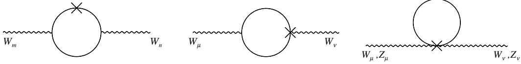
Figure 10: Contribution of the model dependent term \mathcal{L}_\beta to the one loop self-energy of the W and Z gauge bosons.
