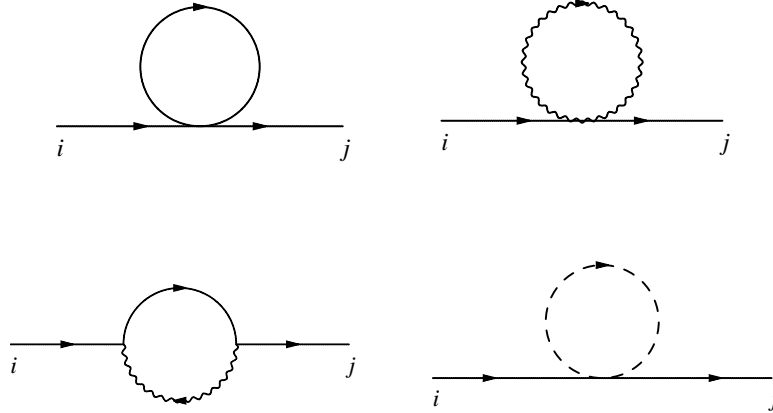
Figure 8: One loop self-energy diagrams for the would-be-Goldstone bosons.
