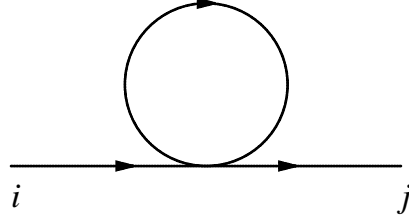
Figure 1: One loop self-energy diagram for the pions.
