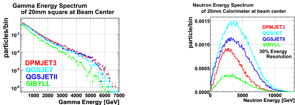
Figure 3. Expected energy spectrum for \gamma s (left) and neutrons (right) according to different interaction models. For neutrons a 30% energy resolution has been taken into account.
