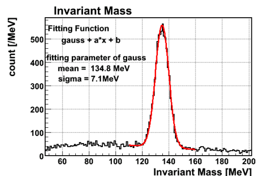
Figure 2. Invariant mass resolution for \pi^0 for the ARM1 calorimeter.
