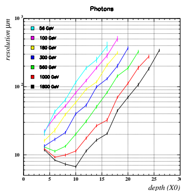
Figure 1. Spatial resolution as a function of layer depth for the ARM2 calorimeter with silicon modules at various photon energies.
