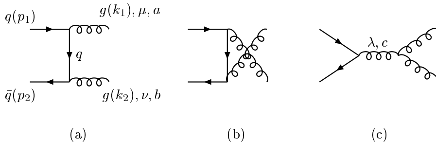
Figure 1: Diagrams contributing to \mathcal{T}_{\mu\nu}^{ab} .
