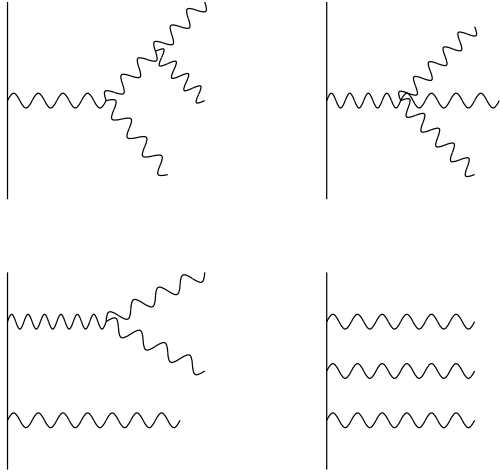
Figure 4: Diagrams contributing to \mathcal{T}_{\mu\nu\rho}^{abc} . We do not show the diagrams which are related to those shown by exchange of outgoing bosons.
