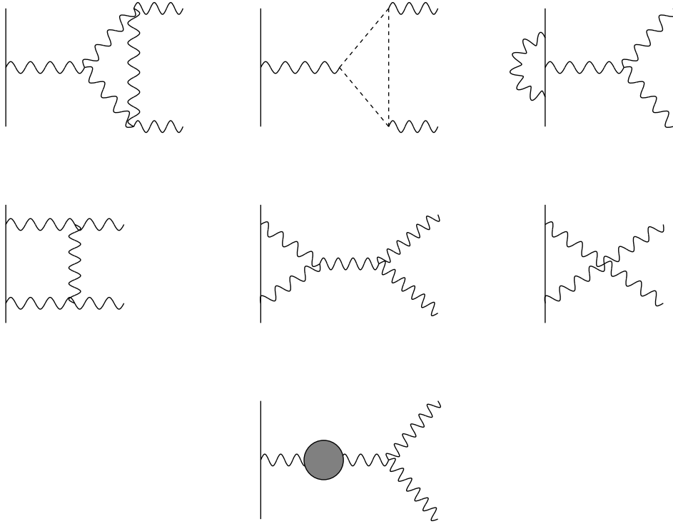
Figure 3: Diagrams contributing to \mathcal{T}_{1\mu\nu}^{ab} . The blob refers to the same corrections to the gluon propagator as in Fig.2(a,e,f).
