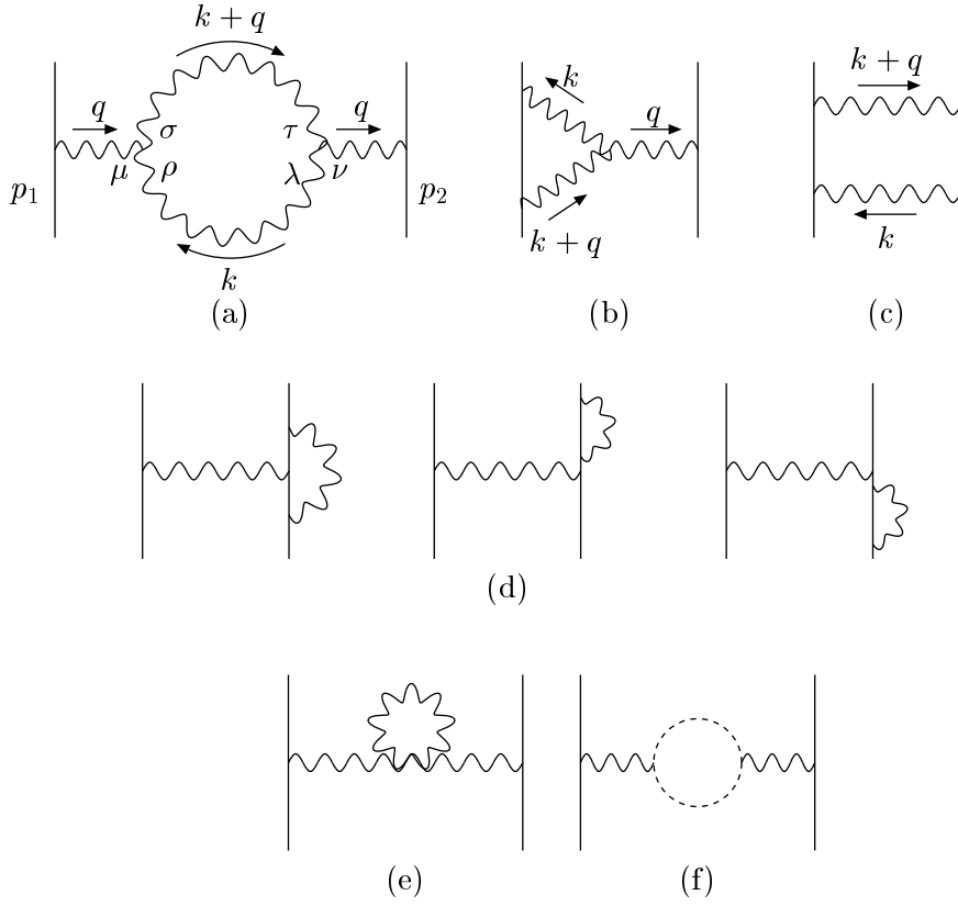
Figure 2: One loop diagrams.
