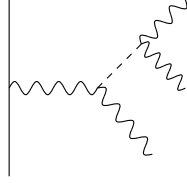
Figure 7: One of the graphs contributing to \mathcal{T}_{\mu\nu\rho}^H . The others are obtained by permuting the outgoing bosons.
