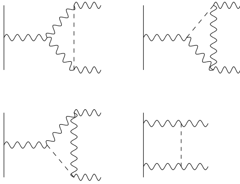
Figure 6: The Higgs graphs contributing to \mathcal{T}_1^H . The graphs of Fig.3 must also be included when computing \mathcal{T}_1^H .
