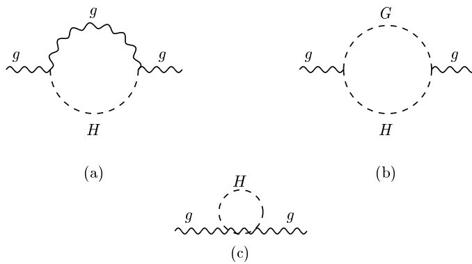
Figure 5: Higgs boson contributions to \widehat{\Pi}_{\mu\nu}^{gH} . In the unitary gauge recall that (b) is absent.
