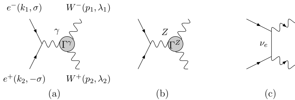
Fig. 1: The process e^+e^- \rightarrow W^+W^- at tree level, including anomalous gauge boson couplings.
