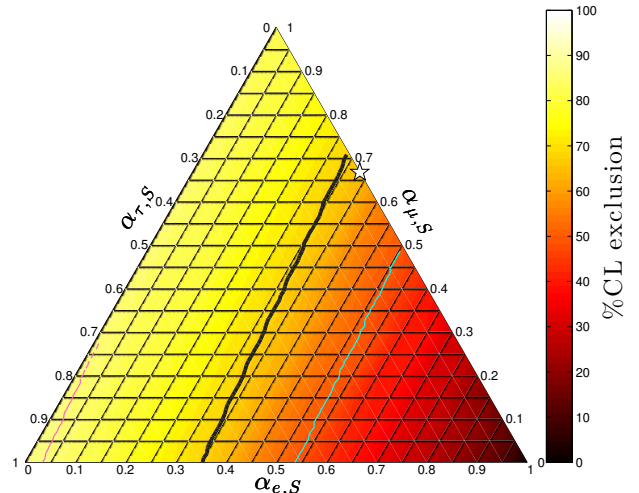
FIG. 2. Same as Fig. 1, but for \{\alpha_{i,S}\} at the source and assuming the signal neutrinos are astrophysical and oscillation probabilities are in the averaged regime, i.e., the parameter space is restricted to the blue sliver shown in Fig. 1. The best-fit is the darkest point, (1 : 0 : 0)_S . The white star corresponds to the (1 : 2 : 0)_S flavor combination. Standard flavor compositions lie within a narrow band along the right side of the triangle. Note that all combinations are allowed at 95% C.L. for the three spectra, and even at 68% C.L. for E_{\nu}^{-3} .
