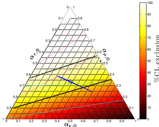
FIG. 1. Ternary plot of the exclusion C.L. for all possible flavor combinations ( \alpha_{e,\oplus} : \alpha_{\mu,\oplus} : \alpha_{\tau,\oplus} ) as seen at Earth, given the 7 tracks and 21 showers observed at IceCube. The lower right corner corresponds to 100% electron neutrinos, the upper corner is 100% muon neutrinos, and the lower left corner to 100% tau neutrinos. The central sliver outlined in blue corresponds to the possible flavor combinations for astrophysical neutrinos, after oscillations have been averaged during propagation. The best-fit is the darkest point, (1 : 0 : 0)_{\oplus} . The white star corresponds to (1 : 1 : 1)_{\oplus} , which is expected from a (1 : 2 : 0)_S combination at the source. The color scale indicates the exclusion C.L. given an E_{\nu}^{-2} spectrum of incoming neutrinos. Solid (dashed) lines show 68% C.L. (95% C.L.) contours, cyan for E_{\nu}^{-1} , thick black for E_{\nu}^{-2} and pink for E_{\nu}^{-3} spectra.
