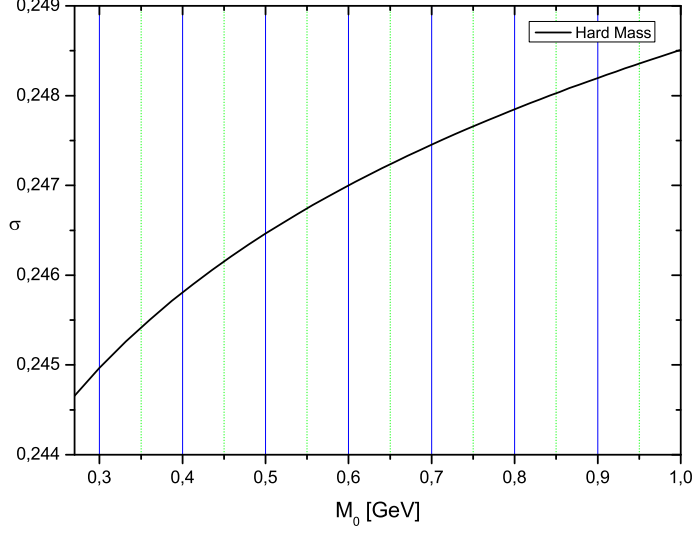
FIG. 6: \sigma as a function of the hard ghost mass M_0 , obtained from Eq.(4.27).
