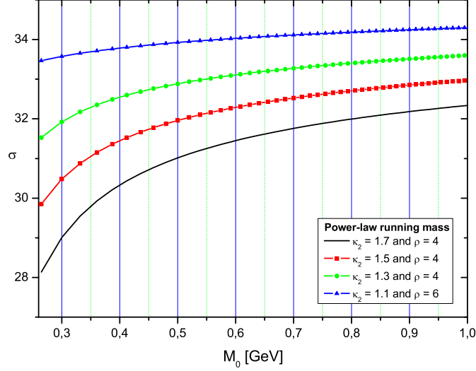
FIG. 8: \sigma as function of M_0 , when the power-law running of Eq.(3.19) is assumed for M^2(k^2) .
