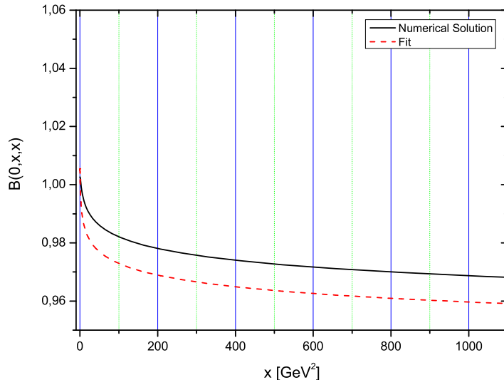
FIG. 5: The black solid line is the numerical solution of Eq.(3.10), assuming logarithmic type of running for m^2(k^2) and M^2(k^2) , with \gamma_1 = \kappa_1 = 0.6 , m_0^2 = 0.35 \text{ GeV}^2 , M_0^2 = 0.4 \text{ GeV}^2 , \rho = 4 , and \sigma^{1/\lambda} = 1 \text{ GeV}^2 . The red dashed line represents the fit of Eq.(3.20); the relative difference between the two curves is less than 1% (note the fine spacing of the y axis).
