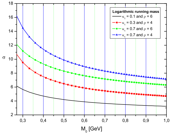
FIG. 7: \sigma as function of M_0 , when M^2(k^2) runs logarithmically, as in Eq.(3.18).
