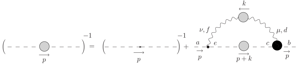
FIG. 1: The SDE of the ghost propagator.
