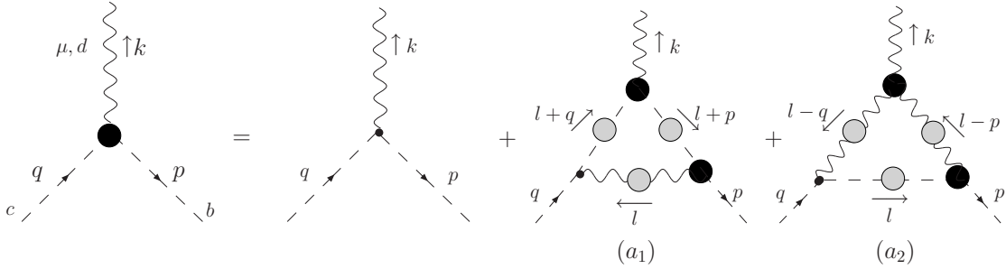
FIG. 3: Truncated version of the SDE for the gluon-ghost vertex.
