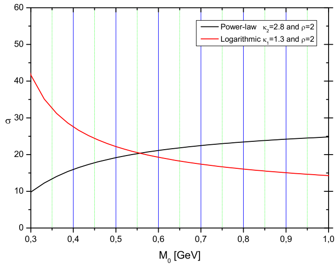
FIG. 9: For \sigma = 20 , a ghost mass can be generated from Eq.(4.24) for either type of running.
