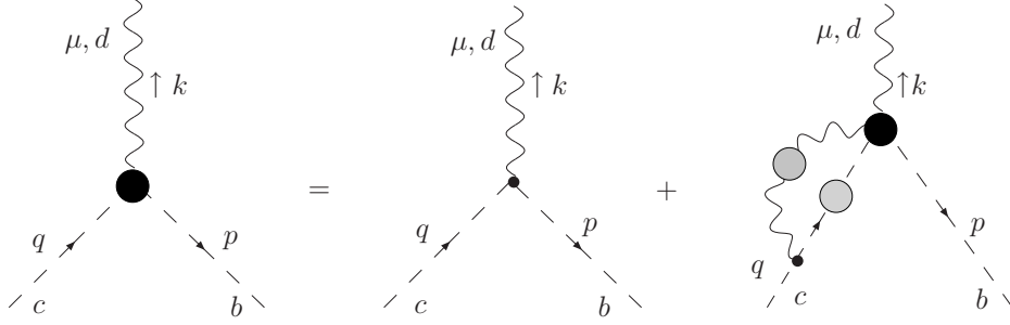
FIG. 2: SDE for the gluon-ghost vertex.
