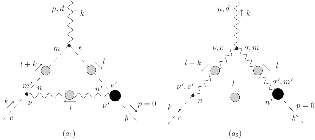
FIG. 4: Contributions for the gluon-ghost vertex equation in the limit of p \rightarrow 0 .
