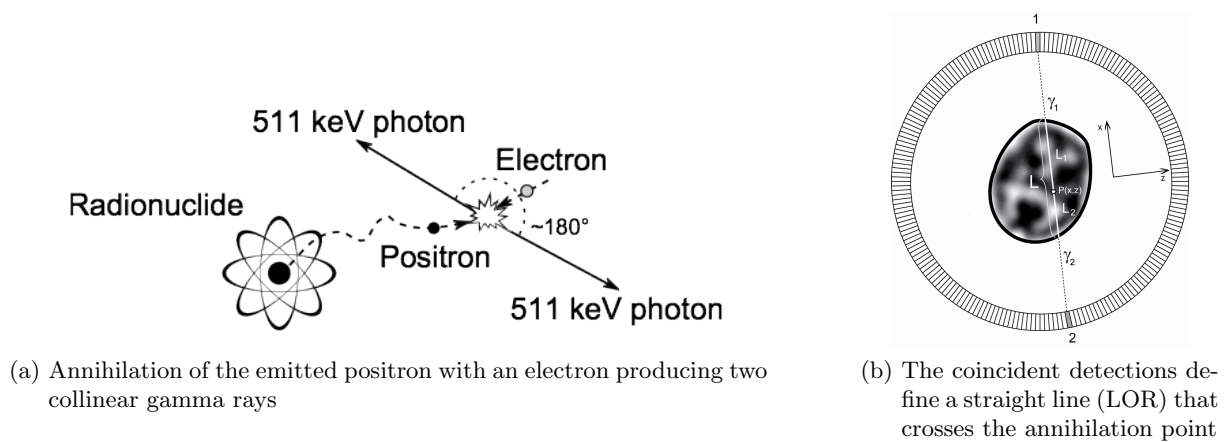
FIG. 2: PET principle
