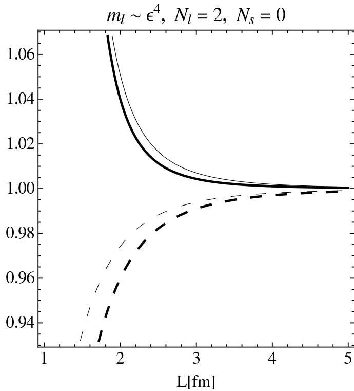
Figure 1: Ratio of \mathcal{C}_j^{(e)l}(t = 1fm) at fixed volume normalised to the \infty volume result as a function of L for two boxes with T = L (solid) and T = 2L (dashed), and for g_\pi = 0.44 (thick lines) [30] and g_\pi = 0 (thin lines). We have fixed \Sigma = (250 \text{ MeV})^3, F = 90 \text{ MeV} .
