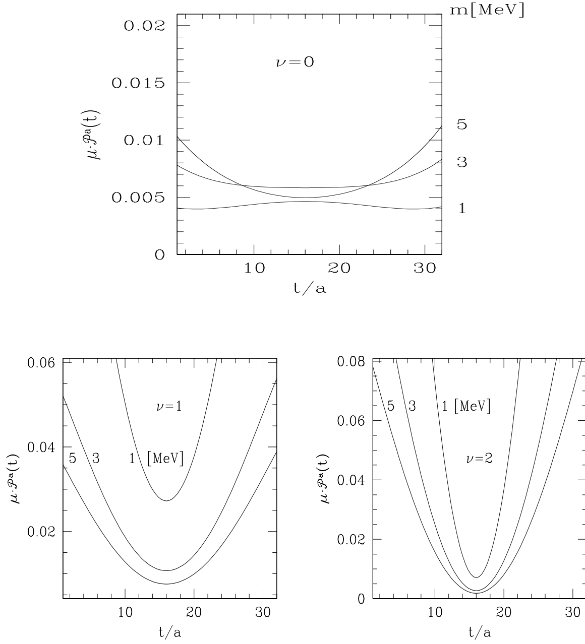
Figure 2: \mu \mathcal{P}^a(t) for quark masses m = 1, 3 and 5 MeV and \nu = 0 (upper), 1 (down left), 2 (down right). The lattice volume is V = L^3 T = 16^3 32 and a^{-1} \simeq 2 GeV.
