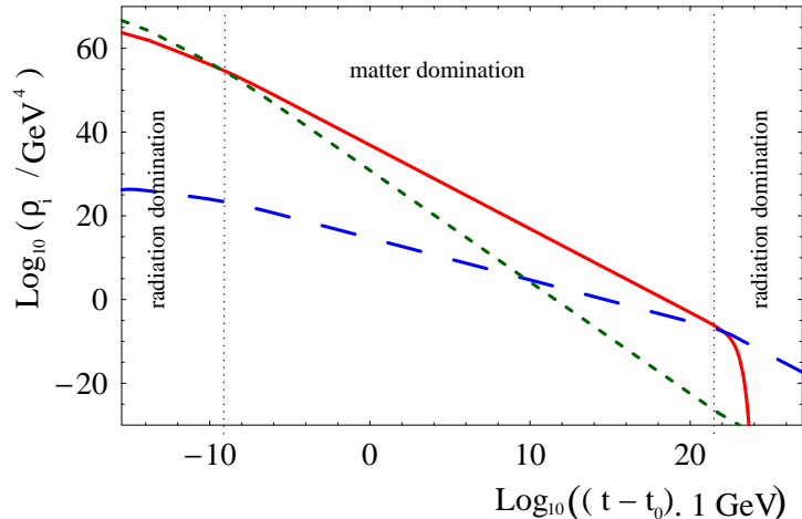
FIG. 1: Evolution of the different components of the energy density of the Universe from T \sim 10^{14} GeV to T \sim 1 MeV. Short-dashed (green) line corresponds to \rho_r^{\text{old}} versus time, long-dashed (blue) line to \rho_r^{\text{new}} and the solid (red) line to \rho_X . We start from \rho_X = \rho_r^{\text{old}}/200 at T \sim 10^{15} GeV, with a \Gamma_X = 10^{-20} GeV.
