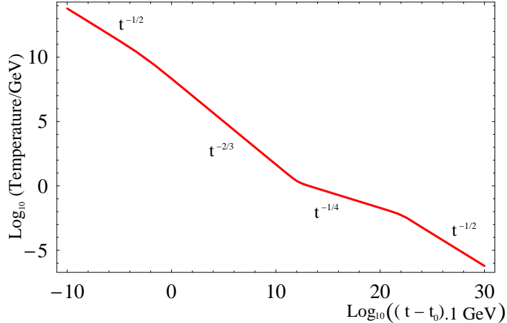
FIG. 2: Temperature of the Universe (in GeVs) as a function of time. The four different epochs in the evolution of the Universe, radiation domination, matter domination, decay and radiation domination again can be seen in the different slopes of the curve. The time dependence of the temperature is explicitly indicated for each epoch.
