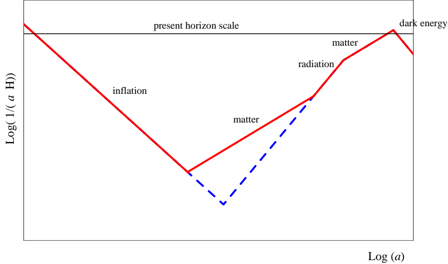
FIG. 3: Comoving Hubble radius, \log(1/aH) , versus \log a . This plot shows the different eras entering the e -foldings calculation. Inflation is an epoch where \log(1/aH) is decreasing. Exponential inflation gives a line with a slope of -1. In all other cases the inflation line is shallower. During matter domination (1/aH) \propto a^{1/2} , while during radiation domination (1/aH) \propto a . The current dark energy domination signals a new inflationary epoch. The horizontal (black) solid line indicates the present horizon scale. The number of e -foldings before the end of inflation at which observable perturbations were born is the horizontal distance between the time when (1/aH) first crosses that value and the end of inflation. The solid (red) line represents a Universe with a period of matter domination before BBN. The dashed (blue) line represents the standard cosmological history of the Universe with only one (recent) epoch of matter domination.
