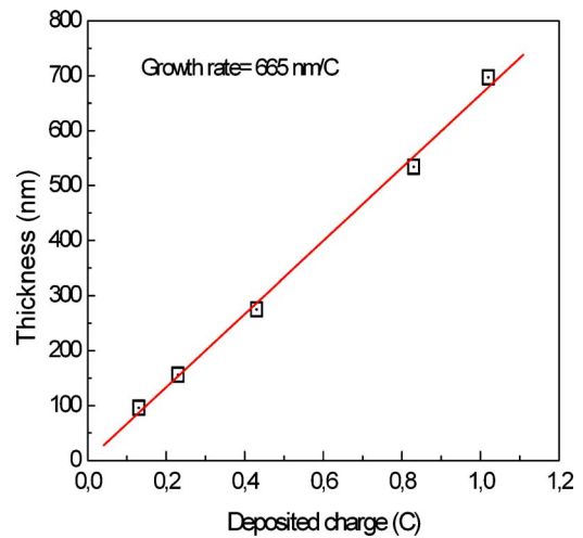
FIG. 4. (Color online) Thickness of several \text{Zn}_{0.83}\text{Co}_{0.17}\text{O} films as a function of the deposited electrical charge.
