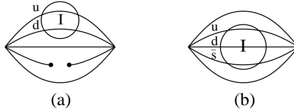
Figure 3: An example of instanton two- and three-body contributions to the correlator of the pentaquark currents.
