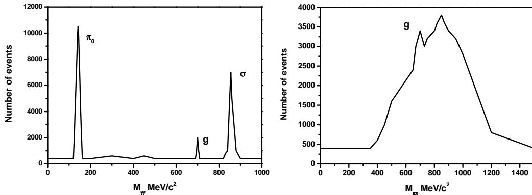
Figure 4: Expected fit to the two-photon invariant mass spectrum and the two-pion invariant mass spectrum in central Pb-Pb collisions after subtraction from the background. The 2\gamma decays should allow for a clear separation of g and \sigma . The 2\pi decays will show the g arising above the \sigma background.
