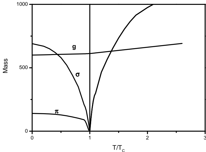
Figure 2: Behavior of the masses of \sigma, \pi and g across the QGP phase transition according to model calculations.
