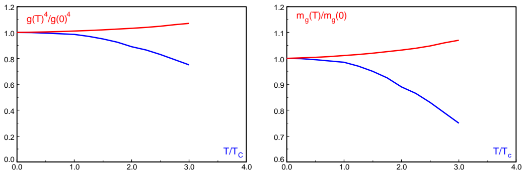
Figure 1: Behavior of the gluon condensate, g^4 = m_g^2 f_g^2 , and the mass, m_g , of g across the de-confinement phase transition for various calculations mentioned in the text. The allowed values for different model calculations occur between the two lines.
