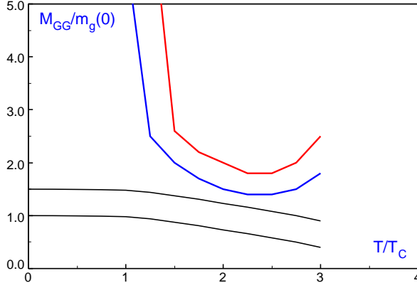
Figure 3: Behavior of the glueball masses as one approaches the de-confinement phase transition. The mass of the color singlet states remains basically constant while the mass of the color states increases dramatically.
