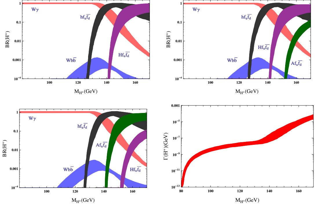
Figure 6: Charged-Higgs branching ratios as functions of M_{H^\pm} , for \lambda_{hH^+H^-} = \lambda_{HH^+H^-} = 1 , \cos \tilde{\alpha} \in [0.9, 0.99] , M_H = 140 GeV, M_A > M_W + M_Z (top-left); (M_H, M_A) = (140, 150) GeV (top-right) and (M_H, M_A) = (150, 140) GeV (bottom-left). The total decay width for the first case is also shown (bottom-right).
