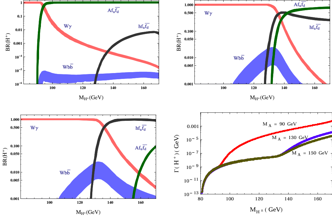
Figure 5: Charged-Higgs branching ratios as functions of M_{H^\pm} , for \lambda_{hH^+H^-} = \lambda_{HH^+H^-} = 1 , \cos \tilde{\alpha} = 0.9 and M_A = 90 (top-left), 130 (top-right) and 150 (bottom-left) GeV. M_H is varied from M_W + M_Z up to its permitted value by the oblique parameters. The bottom-right panel shows the corresponding total decay widths.
