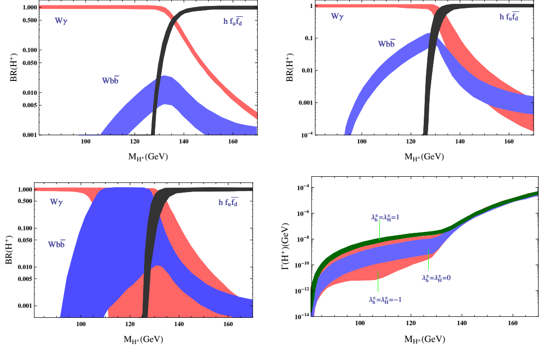
Figure 4: Charged-Higgs branching ratios as functions of M_{H^\pm} \in [M_W, M_W + M_Z] , for \cos \tilde{\alpha} = 0.9 , M_H \in [M_W + M_Z, 500 \text{ GeV}] and \lambda_{hH^+H^-} = \lambda_{HH^+H^-} = 1 (top-left), 0 (top-right) and -1 (bottom-left). The corresponding total decay widths are shown in the bottom-right panel ( \lambda_h^\pm \equiv \lambda_{hH^+H^-} , \lambda_H^\pm \equiv \lambda_{HH^+H^-} ).
