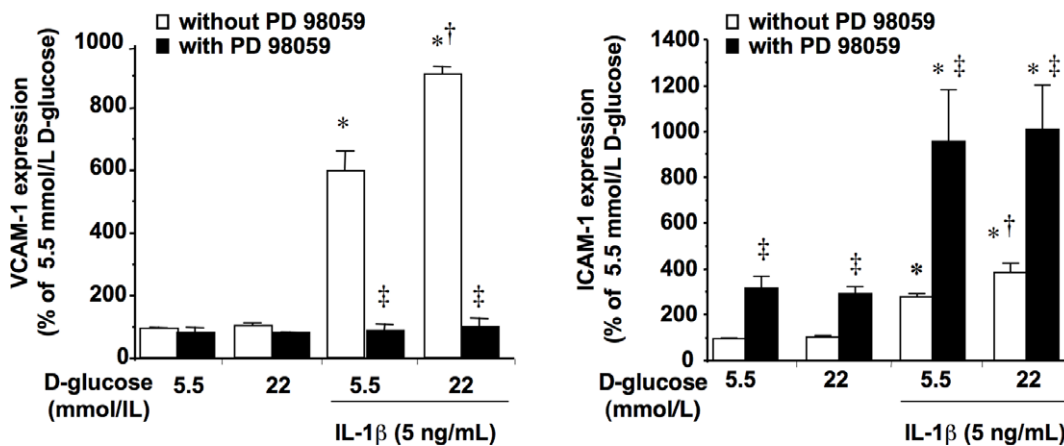
Figure 2. ERK 1/2 activation and its impact on ICAM-1 and VCAM-1 levels in HUVEC. (A) Cells were incubated in medium containing 5.5 mmol/L or 22 mmol/L D-glucose with or without IL-1β (5 ng/mL) for 5–60 min, after which ERK 1/2 activation was determined by Western blotting. Representative gels are shown on the top. (B) Involvement of ERK 1/2 in CAMs expression. HUVEC were cultured for 18 h in the above-described conditions. PD 98059 (30 μmol/L) was used as an inhibitor of ERK 1/2 activation. * P <0.05 versus 5.5 mmol/L D-glucose; † P <0.05 versus 5.5 mmol/L D-glucose in the presence of IL-1β; ‡ P <0.05 versus matched treatment without PD 98059. doi:10.1371/journal.pone.0010091.g002
