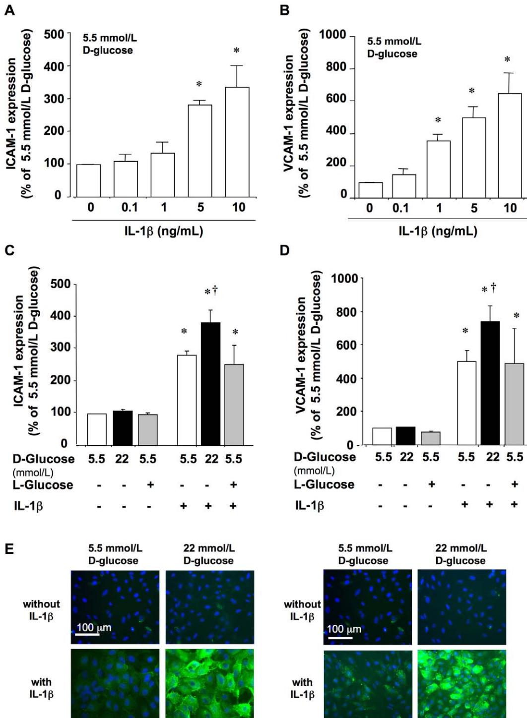
Figure 1. Effect of IL-1β and D-glucose on the expression of adhesion molecules in HUVEC. Cells incubated in a medium containing 5.5 mmol/L D-glucose were challenged for 18 h with IL-1β (0.1 to 10 ng/mL) and the levels of (A) ICAM-1 and (B) VCAM-1 were determined at the cell surface by flow cytometry. In another set of experiments, cells were incubated for 18 h in medium containing 5.5 or 22 mmol/L D-glucose in the presence or absence of IL-1β (5 ng/mL), after which (C) ICAM-1 and (D) VCAM-1 levels were quantified. L-glucose was used as an osmotic control. * P <0.05 versus 5.5 mmol/L D-glucose without IL-1β; † P <0.05 versus 5.5 mmol/L D-glucose with IL-1β. (E) ICAM-1 (left panel) and VCAM-1 (right panel) were visualized by indirect immunofluorescence in HUVEC cultured for 18 h in culture medium containing 5.5 or 22 mmol/L D-glucose in the presence or absence of IL-1β (5 ng/mL). Nuclei were counterstained in blue with 4'-6-diamidino-2-phenylindole (DAPI) (x400). doi:10.1371/journal.pone.0010091.g001
