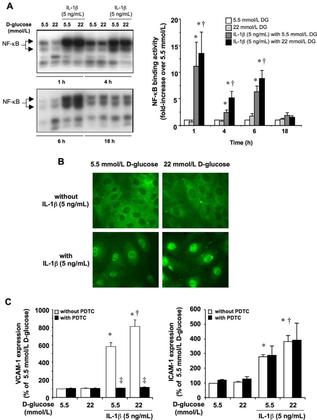
Figure 3. NF- \kappa B activation in HUVEC and its impact on ICAM-1 and VCAM-1 levels. (A) HUVEC were incubated in medium containing 5.5 mmol/L or 22 mmol/L D-glucose in the presence or absence of IL-1 \beta (5 ng/mL) during 1, 4, 6 and 18 h, after which NF- \kappa B binding activity was quantified by EMSA. Representative EMSAs are shown on the left. (B) Translocation of NF- \kappa B from cytoplasm to nucleus was visualized by indirect immunofluorescence in HUVEC cultured for 1 h as mentioned above (x1000). (C) Involvement of NF- \kappa B in CAMs expression. HUVEC were cultured for 18 h in the above-mentioned conditions. PDTC (100 \mu mol/L) was used as NF- \kappa B inhibitor. * P <0.05 versus 5.5 mmol/L D-glucose; † P <0.05 versus 5.5 mmol/L D-glucose with IL-1 \beta ; ‡ P <0.05 versus matched treatment without PDTC. doi:10.1371/journal.pone.0010091.g003
