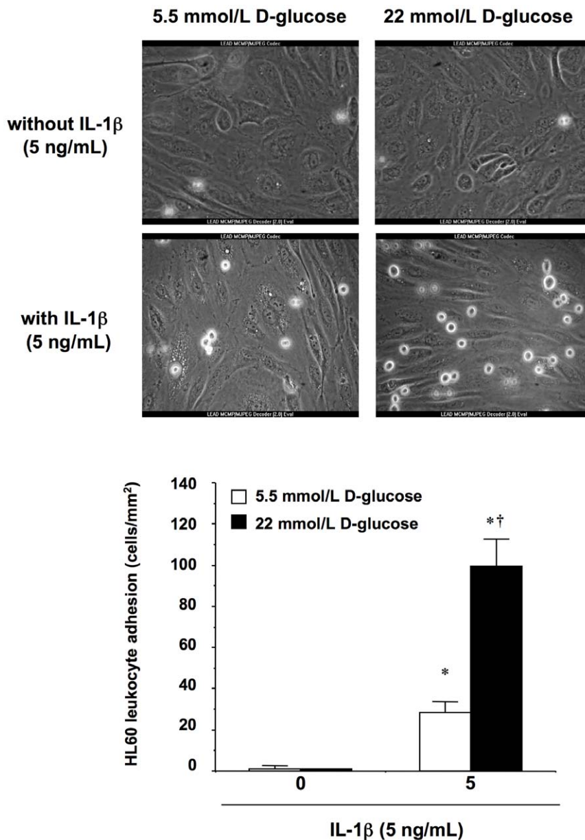
Figure 4. Adhesion of HL60 leukocytes to HUVEC under flow conditions in vitro . HUVEC monolayers were exposed to either 5.5 or 22 mmol/L extracellular D-glucose in the presence or absence of IL-1 \beta (5 ng/mL) for 18 h prior to leukocyte perfusion. * P < 0.05 versus 5.5 mmol/L D-glucose without IL-1 \beta ; † P < 0.05 versus IL-1 \beta in the presence of 5.5 mmol/L D-glucose. Representative micrographs showing HL60 adhesion to HUVEC monolayers are shown on the top (x200).
