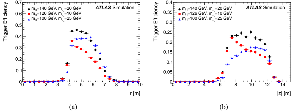
Figure 13: Efficiency for the Muon RoI Cluster trigger as a function of (a) the radial decay position, r , for \pi_{\nu} decays in the barrel and (b) the |z| position for \pi_{\nu} decays in the end-caps.
