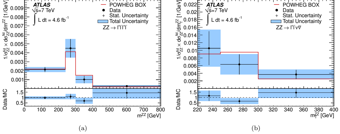
Figure 10. Unfolded ZZ fiducial cross sections in bins of (a) m^{ZZ} for the ZZ \rightarrow \ell^+\ell^-\ell^+\ell^- selection and (b) m_T^{ZZ} for the ZZ \rightarrow \ell^+\ell^-\nu\bar{\nu} selection.
