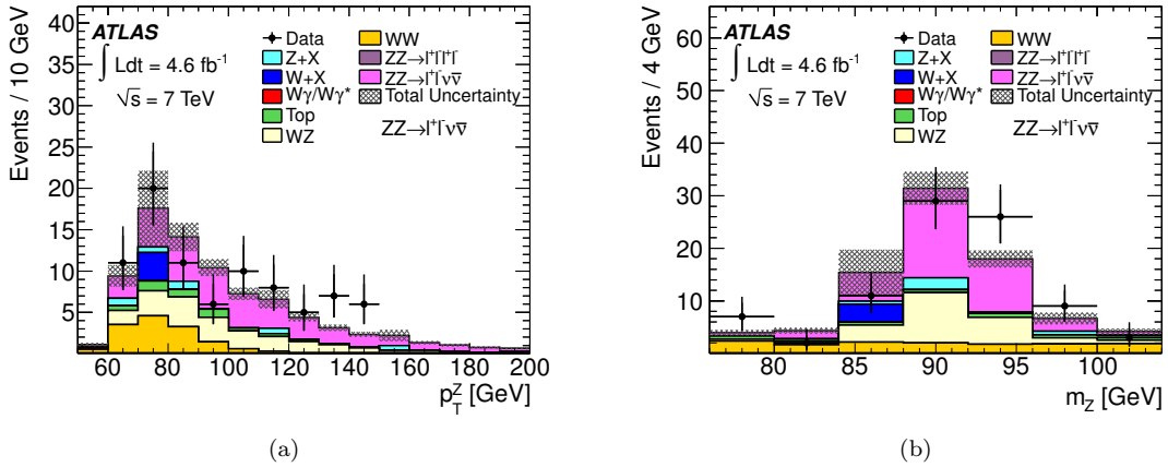
Figure 7. (a) Transverse momentum p_T^Z and (b) mass m_Z of the two-charged-lepton system for the ZZ \rightarrow \ell^+\ell^-\nu\bar{\nu} selection. The points represent the observed data and the histograms show the prediction from simulation. The shaded band shows the combined statistical and systematic uncertainty on the prediction.
