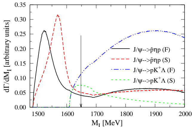
FIG. 3: (Color online) Invariant mass distributions of J/\psi \rightarrow \bar{p}\eta p and J/\psi \rightarrow \bar{p}K^+\Lambda . The theoretical results labeled “F” are obtained using the full U\chi PT amplitudes containing the vertex and \pi\pi N loop corrections, while the ones labeled “S” are obtained by using the amplitudes without these two corrections and with the readjusted subtraction constants by fitting the \pi^- p \rightarrow KY data [14].
