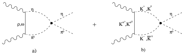
FIG. 4: Loop diagrams for VMD terms. The diagrams with the two crossed photons are not depicted but are also included in the calculations.
