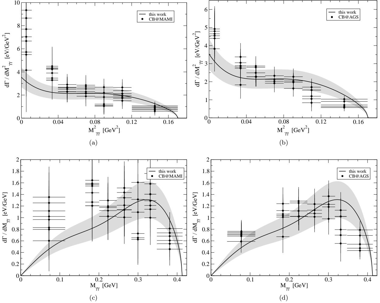
FIG. 7: Two photon invariant mass squared (upper row) and two photon invariant mass (lower row) distributions. The data are from [5] for the Crystal Ball at MAMI (left panels) and for the Crystal Ball at AGS (right panels). The shaded region corresponds to the band of values of the present work considering the theoretical uncertainties.
