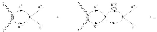
FIG. 3: Resummation for \gamma\gamma \rightarrow \pi^0 \eta .
