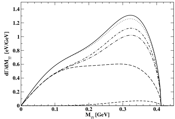
FIG. 6: Contributions to the two photon invariant mass distribution. From bottom to top, short dashed line: chiral loops; long dashed line: only tree level VMD; dashed-dotted line: coherent sum of the previous mechanisms; double dashed-dotted line: idem but adding the resummed VMD loops; continuous line: idem but adding the anomalous terms of Fig. 5, which is the full model presented in this work (we are also showing as a dotted line the full model but substituting the full t_{K^+K^-, \eta\pi^0} amplitude by its lowest order).
