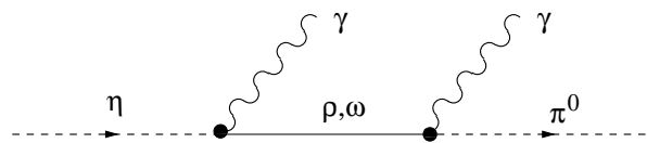
FIG. 1: Diagrams for the VMD mechanism.
