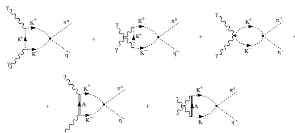
FIG. 2: Diagrams for the chiral loop contribution
