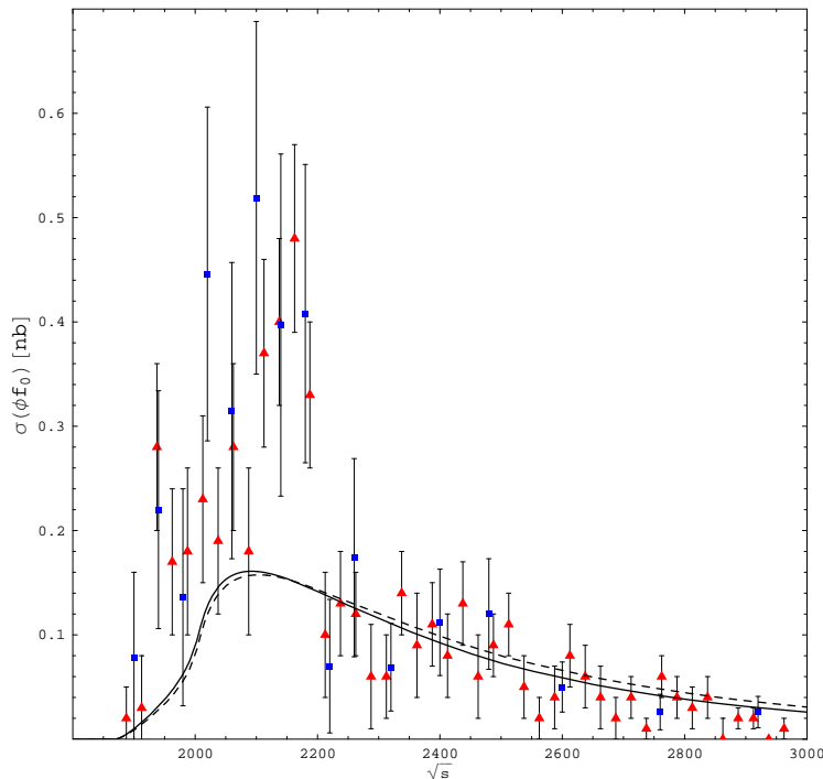
FIG. 4: Cross section for e^+e^- \rightarrow \phi[\pi\pi]_{I=0} , integrated in the m_{\pi\pi} = 850 - 1100 \text{ MeV} range, as a function of \sqrt{s} including all contributions. Experimental points from Ref. [4], triangled (boxed) points correspond to charged (neutral) pions.
