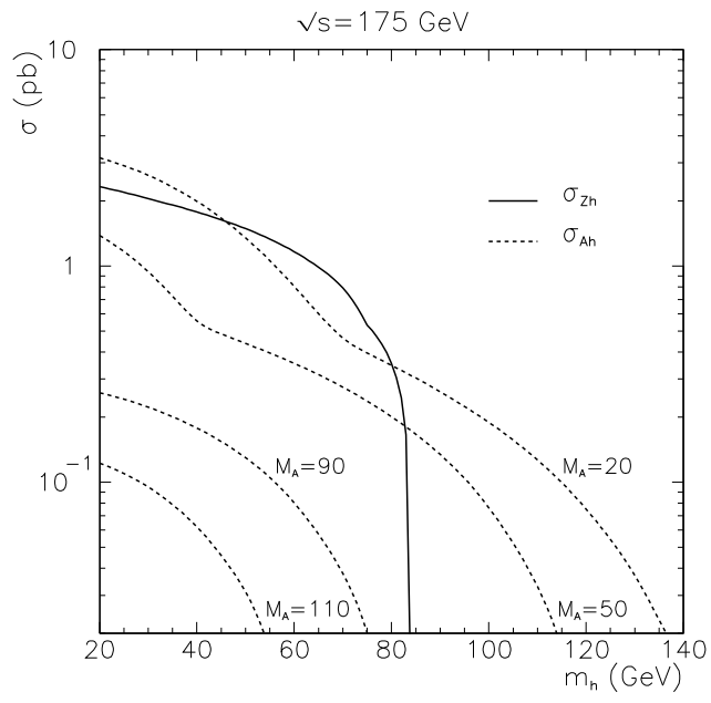
Figure 1: Total cross section for the production of invisibly decaying Higgs bosons through the Bjorken (solid line) and associated production (dotted line) mechanisms at \sqrt{s} = 175 GeV.
