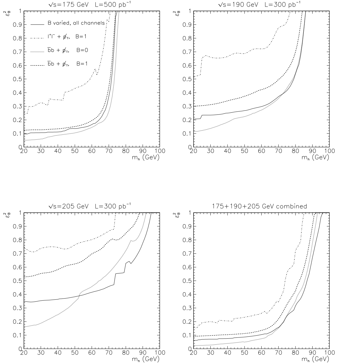
Figure 3: Bounds on \epsilon_B^2 as a function of M_h for three values of \sqrt{s} and the three center-of-mass energies combined. See text for further details.
