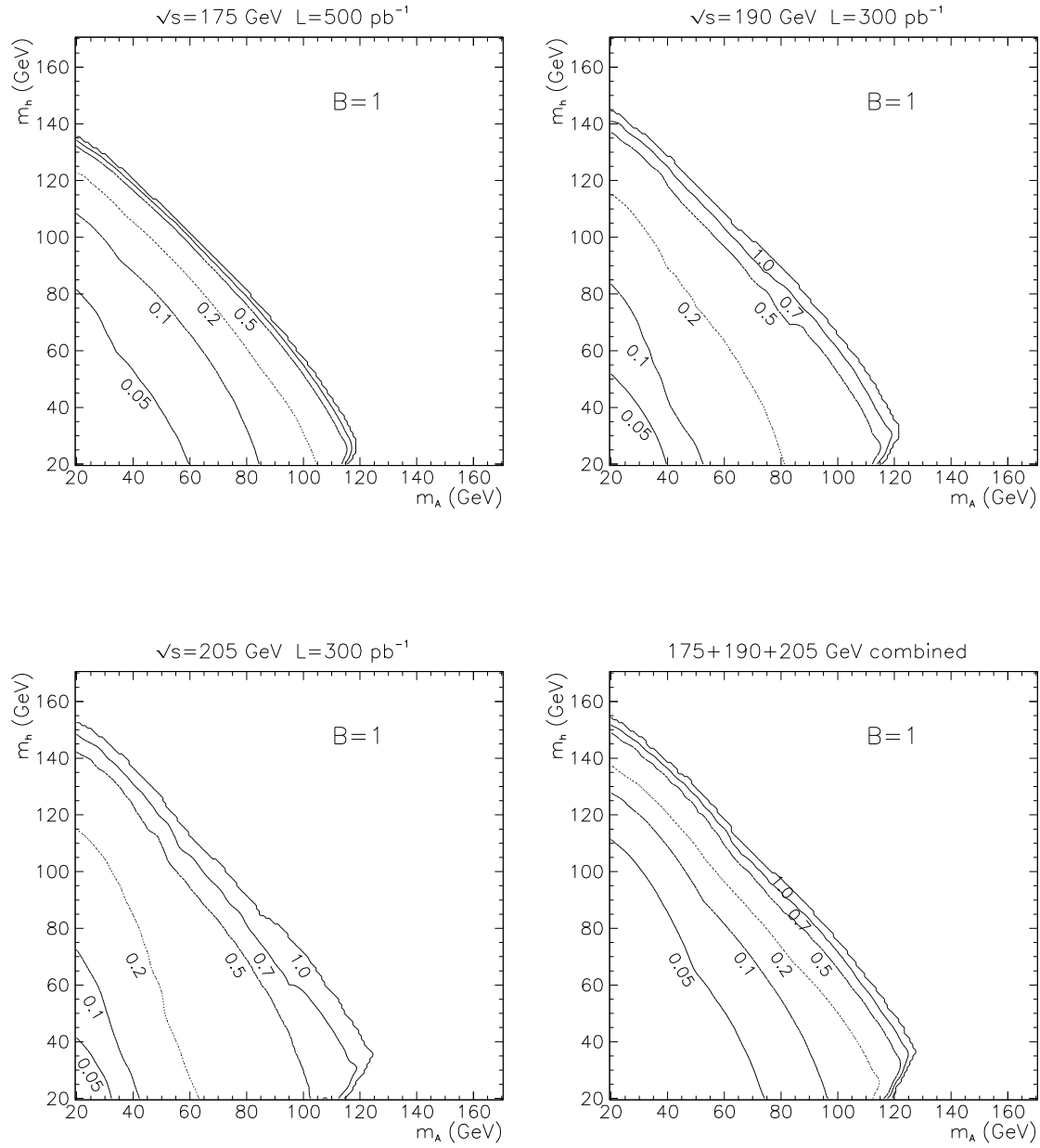
Figure 4: Bounds on \epsilon_A^2 as a function of M_h and M_A for B = 1 . The plots show the bounds obtained for \sqrt{s} = 175, 190, and 205 GeV and the constraints obtained by combining all three expected LEP II runs. The allowed region of the parameter space is above the lines of constant \epsilon_A .
