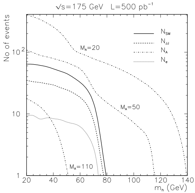
Figure 2: Expected number of signal events after cuts for the processes e^+e^- \rightarrow (Z \rightarrow b\bar{b})+(h \rightarrow JJ) ( N_{JJ} ), e^+e^- \rightarrow (Z \rightarrow \nu\bar{\nu})+(h \rightarrow b\bar{b}) ( N_{SM} ), e^+e^- \rightarrow (A \rightarrow b\bar{b})+(h \rightarrow JJ) ( N_A ), and e^+e^- \rightarrow (Z \rightarrow e^+e^-)+(h \rightarrow b\bar{b}) ( N_e ), assuming \epsilon_A = \epsilon_B = 1 and no suppression due to h decay branching ratios in each case. Note that N_A is given for three choices of M_A values.
