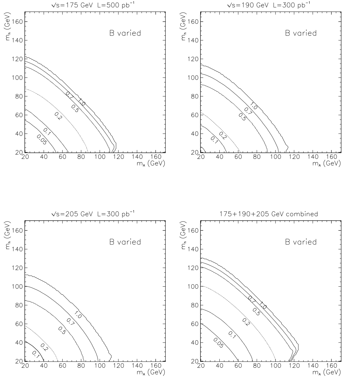
Figure 5: B -independent bounds on \epsilon_A^2 as a function of M_h and M_A . The plots show the constraints obtained for \sqrt{s} = 175, 190, and 205 GeV and the combined bounds from all three expected LEP II runs.
