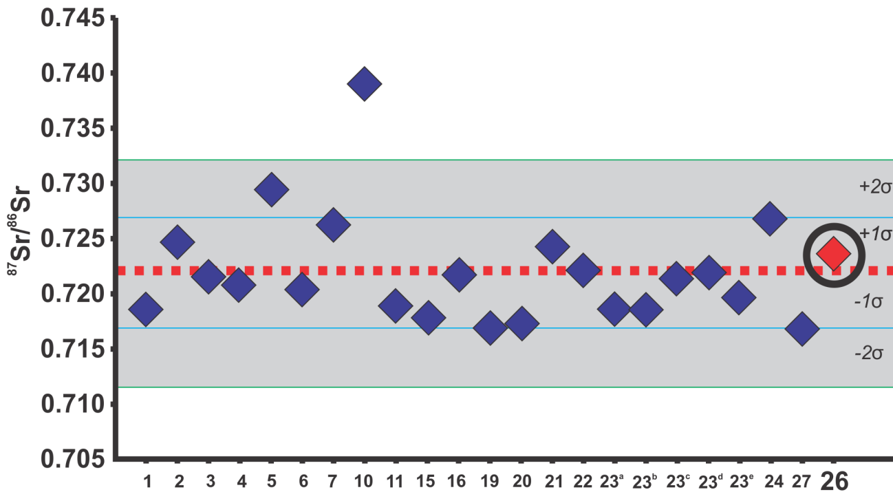
Fig 13. Strontium isotopic analysis. ^{87}\text{Sr}/^{86}\text{Sr} ratio enamel values from the individuals of Lapa do Santo, plotted on ^{87}\text{Sr}/^{86}\text{Sr} mean ratio value (red dashed line), mean ratio \pm 1\sigma values (area between blue lines), and mean ratio \pm 2\sigma values (area between green lines) of the entire sample. A black circle marks the decapitated individual.
