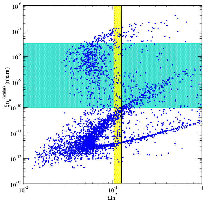
Figure 4: Sneutrino–nucleon scattering cross section \xi \sigma_{\text{nucleon}}^{(\text{scalar})} vs. the sneutrino relic abundance \Omega h^2 , for the same scan of the supersymmetric parameter space given in Fig. 3. The horizontal [light blue] band denotes the current sensitivity of direct detection experiments; the vertical [yellow] band delimits the 3 \sigma C.L. WMAP cold dark matter range [7].
