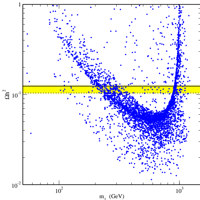
Figure 3: Sneutrino relic abundance \Omega h^2 as a function of the LSP sneutrino mass m_1 , for a full scan of the supersymmetric parameter space: 100 \text{ GeV} < m_0 < 3 \text{ TeV} , 100 \text{ GeV} < m_{1/2} < 3 \text{ TeV} , 1 \text{ GeV}^2 < B_\mu < 100 \text{ GeV}^2 , A_0 = 0 , 3 < \tan \beta < 50 , 10^{-9} \text{ GeV} < \mu_S < 10^{-6} \text{ GeV} . The yellow band delimits the WMAP [7] cold dark matter interval at 3 \sigma of C.L.: 0.104 \leq \Omega_{\text{CDM}} h^2 \leq 0.124 .
