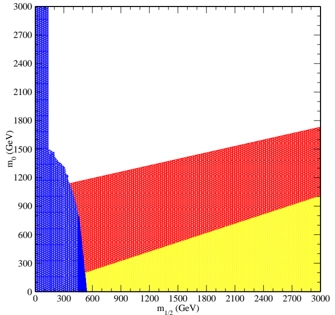
Figure 2: The m_0 - m_{1/2} plane for \tan\beta = 35 , A_0 = 0 and \mu > 0 . The red and yellow areas denote the set of supersymmetric parameters where the sneutrino is the LSP in inverse seesaw models (notice that it includes all the yellow region where the \tilde{\tau} is the LSP in the standard mSUGRA case). The white region has the neutralino as LSP in both standard and modified mSUGRA. For the sneutrino LSP region, the additional parameters are: B_{\mu_S} = 10 \text{ GeV}^2 , M_R = 500 \text{ GeV} , m_D = 50 \text{ GeV} and \mu_S = 1 \text{ eV} . The blue region is excluded (see text).
