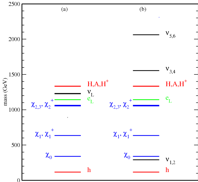
Figure 1: Supersymmetric particle spectrum in the standard MSUGRA scheme [panel (a)] and in the inverse seesaw mSUGRA model [panel (b)] with parameters chosen as: m_0 = 358 GeV, m_{1/2} = 692 GeV, A_0 = 0 , \tan\beta = 35 and sign \mu > 0 . The sneutrino sector has the additional parameter B_{\mu_S} , fixed at 10 \text{ GeV}^2 . The squark sector is not shown.
