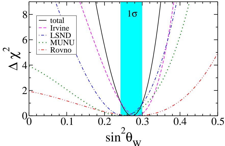
FIG. 2: \Delta\chi^2 for \sin^2\theta_W from \nu_e e or \bar{\nu}_e e scattering. The contribution of each experiment to the \Delta\chi^2 is also shown.
