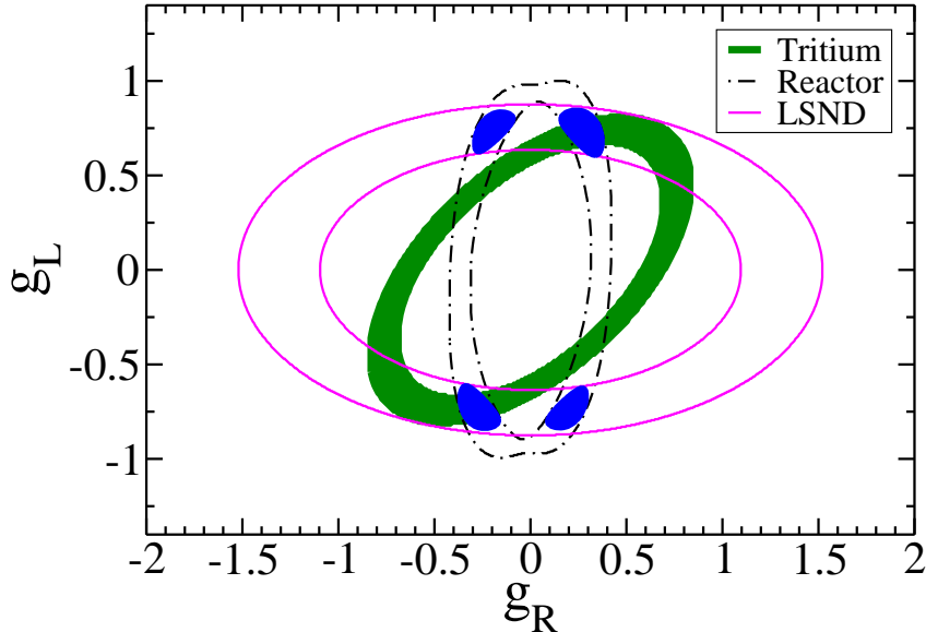
FIG. 1: Allowed 90 % C. L. regions for g_L and g_R obtained by a global fit to neutrino and anti-neutrino electron scattering data. It is possible to see the existence of four allowed regions. The plot also shows the contribution from LSND neutrino electron scattering (horizontal ellipse) and combined data from reactor experiments (vertical ellipse). The tiled ellipse illustrates the potential of a future low-energy artificial neutrino source (Tritium proposal in Ref. [17]).
