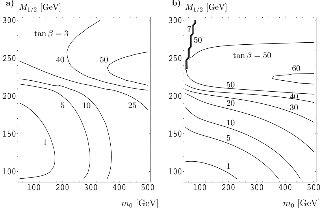
Figure 10: Branching ratios for \tilde{\chi}_1^0 \rightarrow \tau^\pm q \bar{q}' in % in the m_0 - M_{1/2} plane for a) \tan\beta = 3 , and b) \tan\beta = 50 . Here q is the sum over u, d, s , and c . The R-parity violating parameters are fixed such that m_{\nu_3} = 0.06 GeV.
