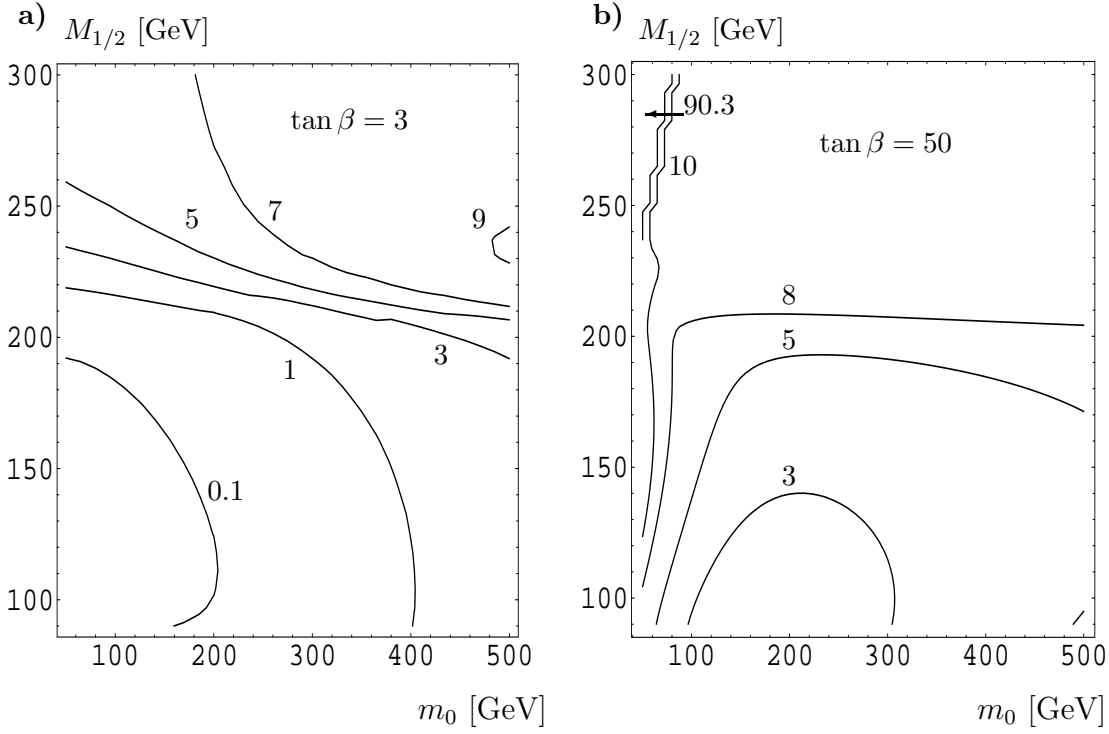
Figure 12: Branching ratios for \tilde{\chi}_1^0 \rightarrow \nu_3 \tau^+ \tau^- in % in the m_0 - M_{1/2} plane for a) \tan \beta = 3 , and b) \tan \beta = 50 . The R-parity violating parameters are fixed such that m_{\nu_3} = 0.06 GeV.
