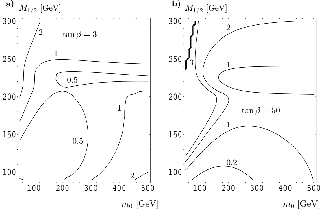
Figure 7: Branching ratios for \tilde{\chi}_1^0 \rightarrow \nu_3 l^+ l^- in % in the m_0 - M_{1/2} plane for a) \tan \beta = 3 , and b) \tan \beta = 50 . Here l is the sum of e and \mu . The R-parity violating parameters are fixed such that m_{\nu_3} = 0.06 GeV.
