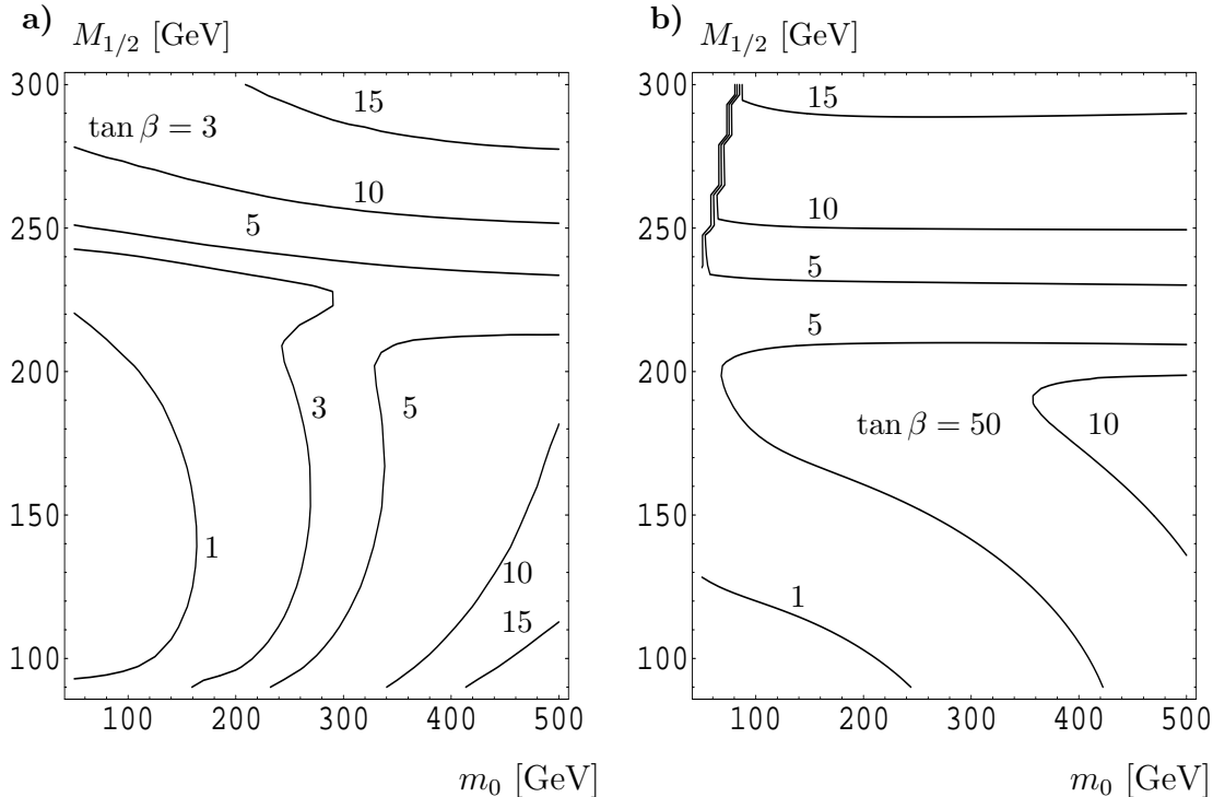
Figure 8: Branching ratios for \tilde{\chi}_1^0 \rightarrow \nu_3 q \bar{q} in % in the m_0 - M_{1/2} plane for a) \tan\beta = 3 , and b) \tan\beta = 50 . Here q is the sum over u , d , s , and c . The R-parity violating parameters are fixed such that m_{\nu_3} = 0.06 GeV.
