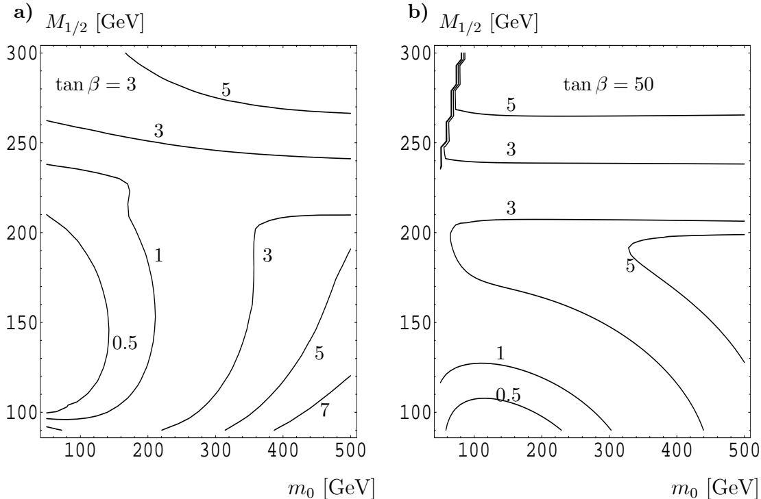
Figure 6: Branching ratios for \tilde{\chi}_1^0 \rightarrow 3\nu in % in the m_0 - M_{1/2} plane for a) \tan\beta = 3 , and b) \tan\beta = 50 . The R-parity violating parameters are fixed such that m_{\nu_3} = 0.06 GeV.
