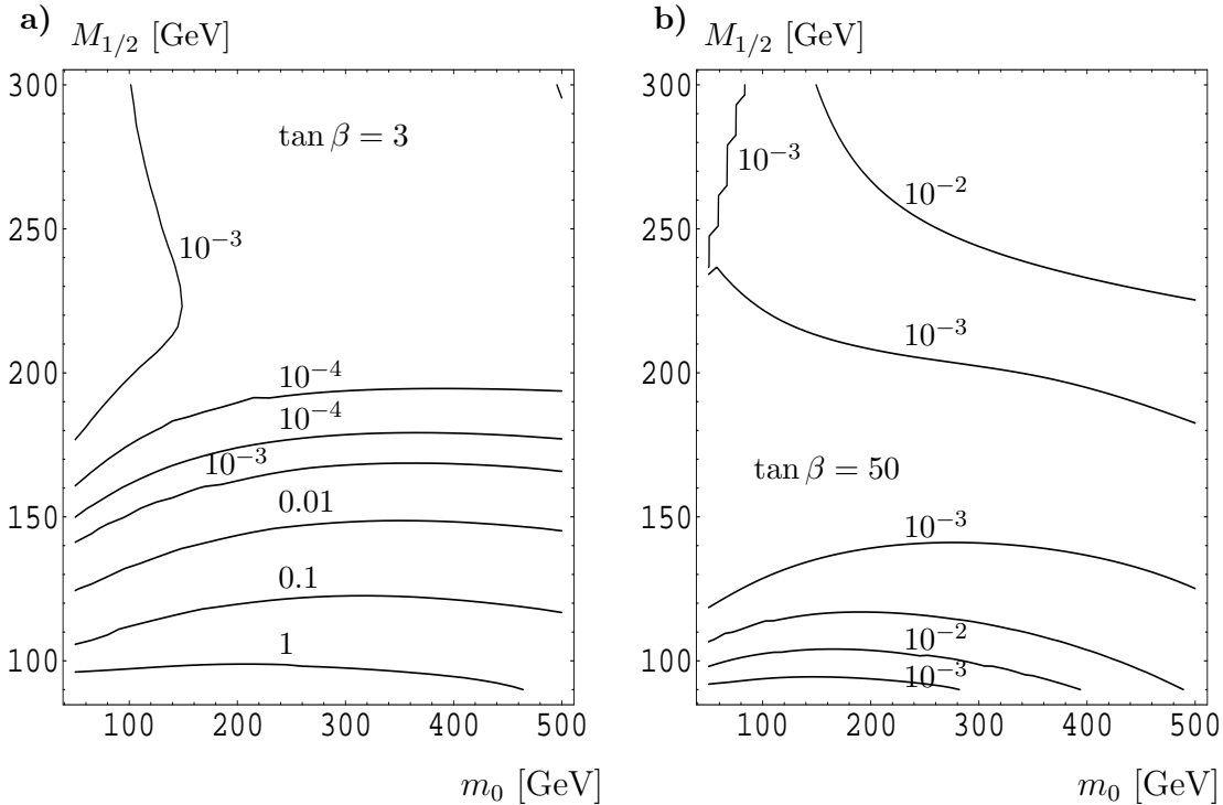
Figure 13: Branching ratios for \tilde{\chi}_1^0 \rightarrow \nu_3 \gamma in % in the m_0 - M_{1/2} plane for a) \tan \beta = 3 , and b) \tan \beta = 50 . The R-parity violating parameters are fixed such that m_{\nu_3} = 0.06 GeV.
