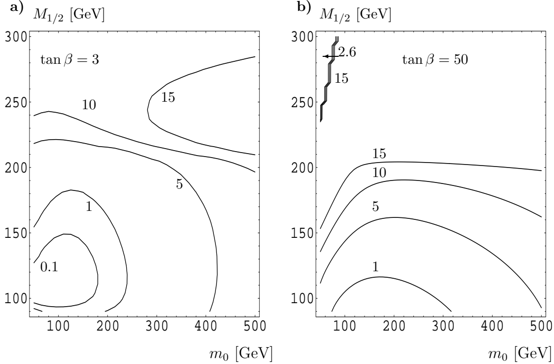
Figure 9: Branching ratios for \tilde{\chi}_1^0 \rightarrow \nu_l \tau^\pm l^\mp in % in the m_0 - M_{1/2} plane for a) \tan \beta = 3 , and b) \tan \beta = 50 . Here l is the sum of e and \mu . The R-parity violating parameters are fixed such that m_{\nu_3} = 0.06 GeV.
