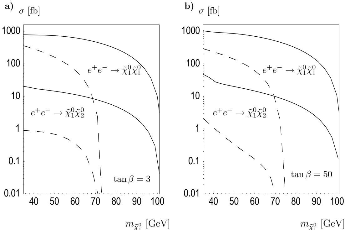
Figure 1: Maximum and minimum attainable values for the e^+e^- \rightarrow \tilde{\chi}_1^0\tilde{\chi}_1^0 (full lines) and e^+e^- \rightarrow \tilde{\chi}_1^0\tilde{\chi}_2^0 (dashed lines) production cross sections in fb as a function of m_{\tilde{\chi}_1^0} for \sqrt{s} = 205 GeV, 50 \text{ GeV} < m_0 < 500 \text{ GeV} , 90 \text{ GeV} < M_{1/2} < 270 \text{ GeV} , a) \tan\beta = 3 , and b) \tan\beta = 50 . ISR corrections are included.
