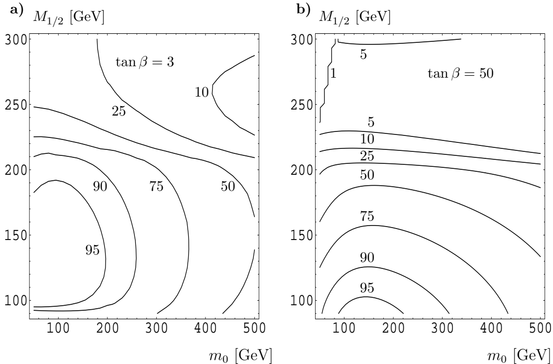
Figure 11: Branching ratios for \tilde{\chi}_1^0 \rightarrow \nu_3 b \bar{b} in % in the m_0 - M_{1/2} plane for a) \tan\beta = 3 , and b) \tan\beta = 50 . The R-parity violating parameters are fixed such that m_{\nu_3} = 0.06 GeV.
