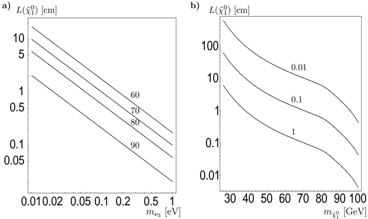
Figure 4: Decay length of the lightest neutralino in cm for \sqrt{s} = 205 GeV, a) as a function of m_{\nu_3} for m_{\tilde{\chi}_1^0} = 60, 70, 80, and 90 GeV, b) as a function of m_{\tilde{\chi}_1^0} for m_{\nu_3} = 0.01, 0.1, and 1 eV.
