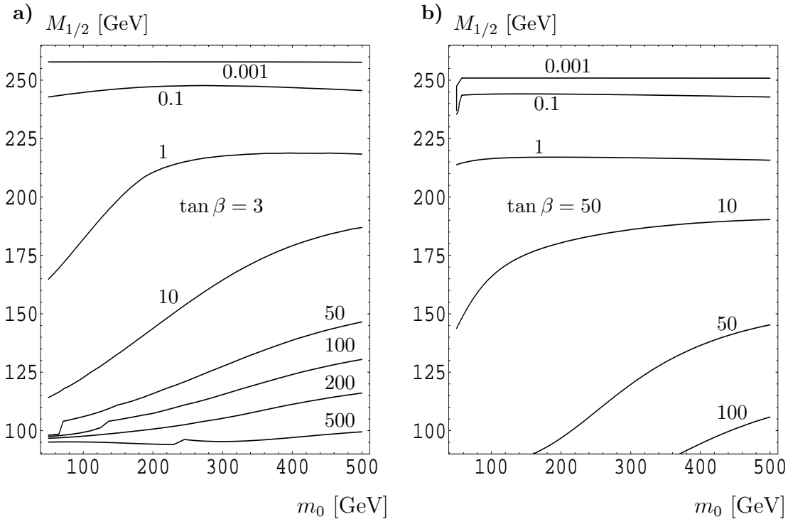
Figure 5: Decay length of the lightest neutralino in cm in the m_0 - M_{1/2} plane for \sqrt{s} = 205 GeV, a) \tan \beta = 3 , and b) \tan \beta = 50 . The R-parity violating parameters are fixed such that m_{\nu_3} = 0.06 GeV.
