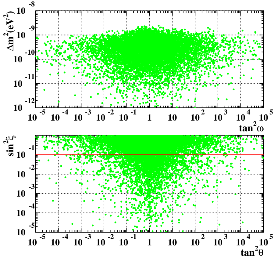
Figure 2: 10000 values of \Delta m_{\odot}^2 and \tan^2 \omega (top), and \sin^2 \xi \tan^2 \theta (bottom) obtained by randomly generated elements for the M_1 matrix and U_{e3} , U_{\mu3} , for m_3 = 0.05 eV (see text). The solid line indicates \sin^2 \xi = 0.1 , which is a good approximation for the upper bound on |U_{e3}|^2 from reactor, solar and atmospheric neutrino data [9].
