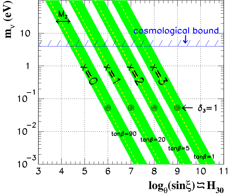
Figure 1: Tree-level neutrino mass dependence on \log_\theta \sin \xi \approx H_{30} for different assignments of the charge difference H_{30} = H_3 - H_0 and for different values of \tan \beta . Details in the text.
