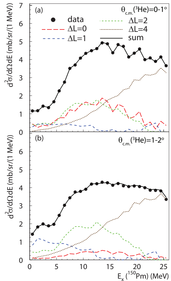
FIG. 8: (color online) MDA results for the 0^\circ - 1^\circ and 1^\circ - 2^\circ angular bins in the {}^{150}\text{Sm}(t, {}^3\text{He}) experiment. Contributions from \Delta L = 2 and \Delta L = 4 transitions are strongly biased due to the absence of a \Delta L = 3 component in the MDA (see text). In both (a) and (b), the results in each 1-MeV wide bin from the MDA for each multipole are connected by lines, rather than showing the individual points.
