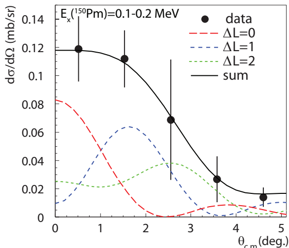
FIG. 10: (color online) Results of MDA fit for the 0.1-0.2 MeV excitation energy bin in ^{150}\text{Sm}(t, ^3\text{He})^{150}\text{Pm} . The \Delta L = 0 angular distribution at 0^\circ has a cross section of 0.08 \text{ mb/sr} \pm 0.03 \text{ mb/sr} . The error bars on the data points are due to statistical errors and systematic errors in the subtraction of background (see Section II B).
