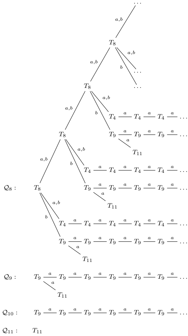
Figure 12: Trees of chains of trees of languages of Example 3.16 (continued)
