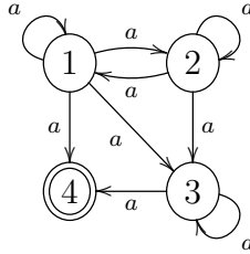
Figure 1: Automaton of Example 3.1
