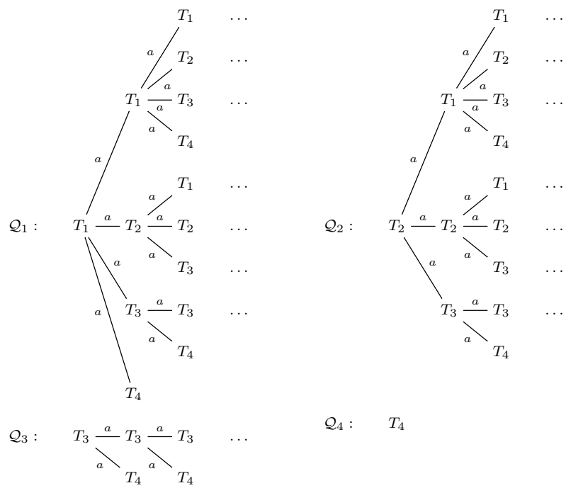
Figure 6: Images of the states in the final automaton \mathcal{L} of the automaton of Example 3.15
