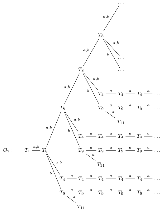
Figure 11: Trees of chains of trees of languages of Example 3.16 (continued)
