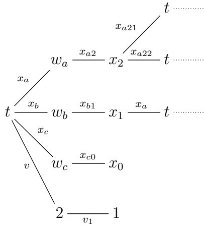
Figure 14: Example of a node of the final realisation for an automaton
