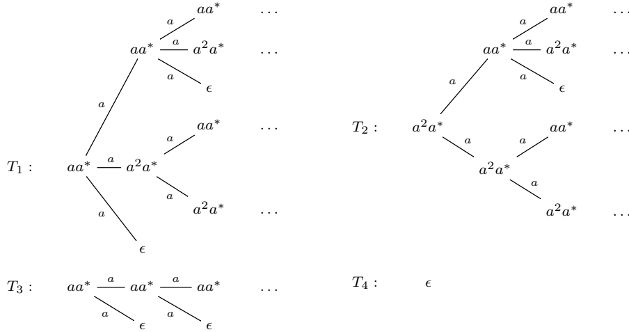
Figure 5: Language trees of the automaton of Example 3.15
