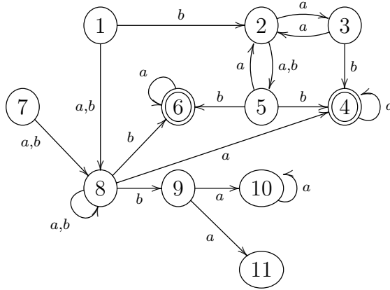
Figure 7: Automaton of Example 3.16
