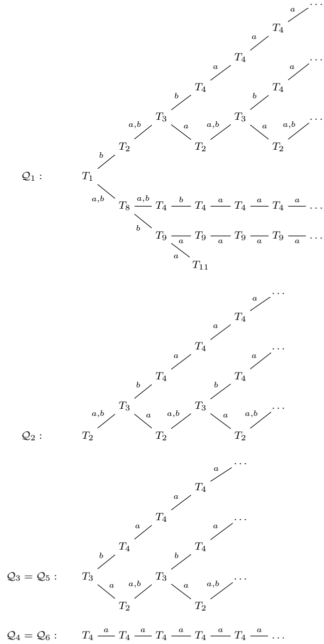
Figure 10: Trees of chains of trees of languages of Example 3.16
