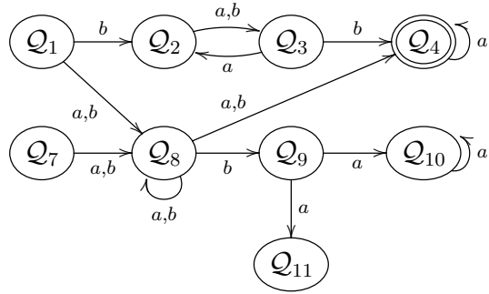
Figure 13: Image of the automaton of Example 3.16 in the final automaton
