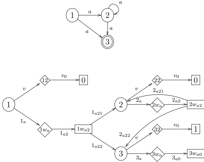
Figure 3: The realisation of an automaton from its graph
