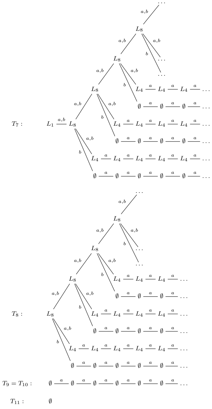
Figure 9: Language sequences of Example 3.16 (continued)
