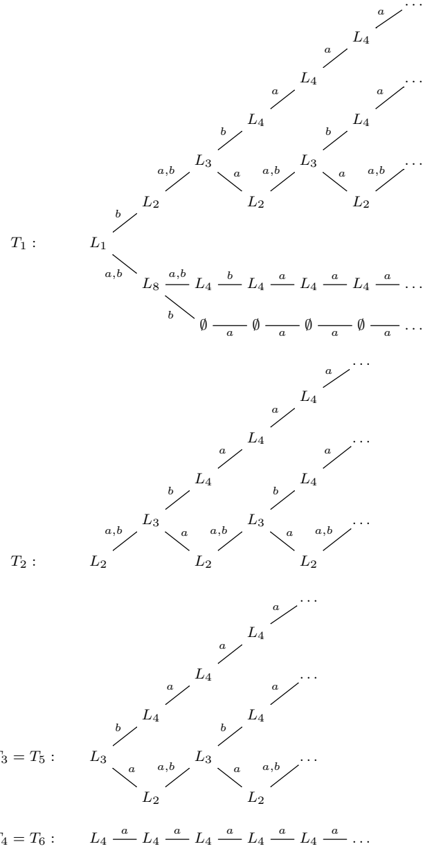
Figure 8: Language sequences of Example 3.16
