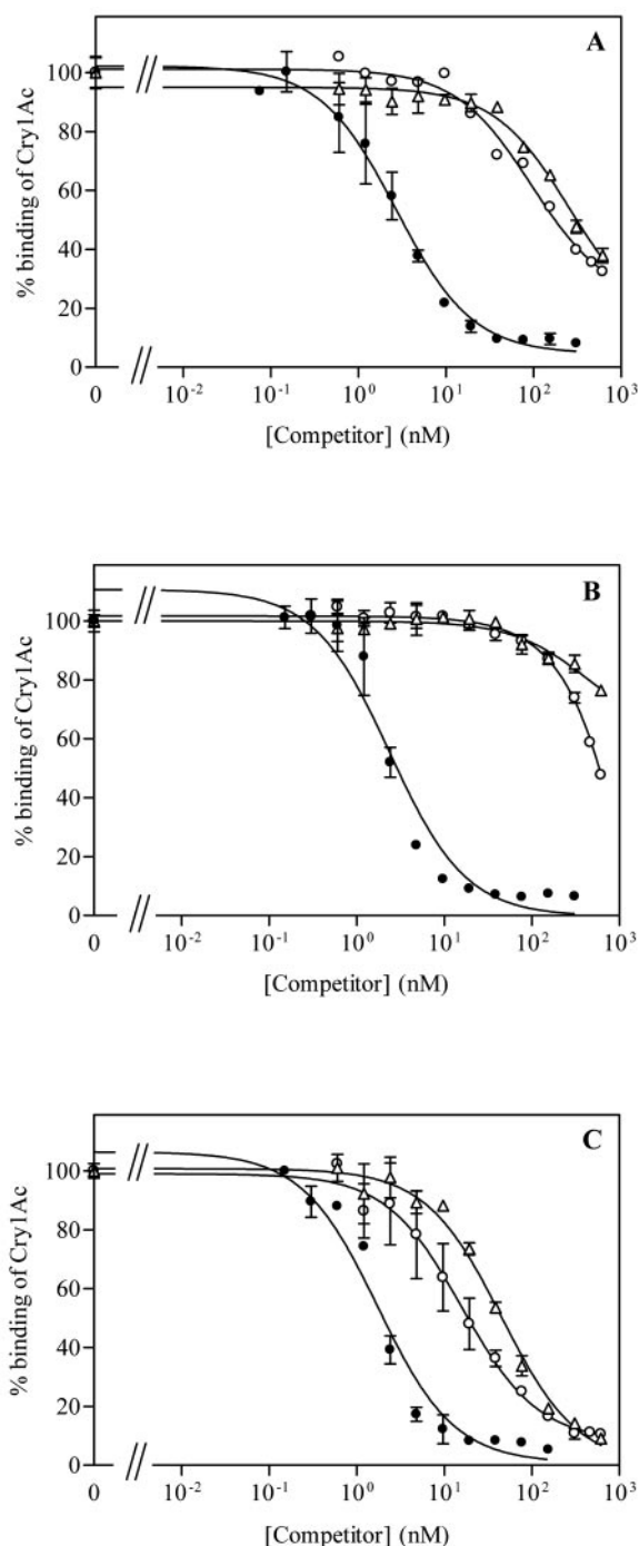
FIG. 1. Binding competition between ^{125}\text{I} -Cry1Ac and increasing concentrations of unlabeled Cry1Ac (●), Cry1Fa (○), or Cry1Ja (△) to BBMV proteins from H. armigera (A), H. zea (B), and S. exigua (C). Each data point is the mean of two independent replications.
