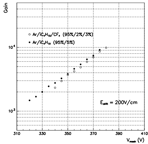
Fig. 4. Left: charge spectrum obtained with a Fe55 X ray source showing a resolution of 10 %. Right: gain versus micromesh high voltage in Ar-iC 4 H 10 (5%) (black dots) and Ar-CF 4 (3%)-iC 4 H 10 (2%) (open circles).
